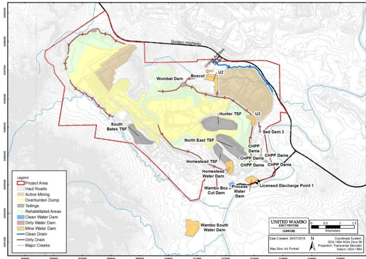
Figure 9-2: Proposed Stage 2 Water Management Structures
