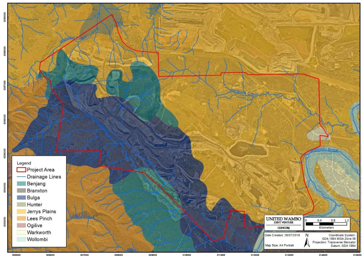
Figure 7-3: Soil Landscapes
