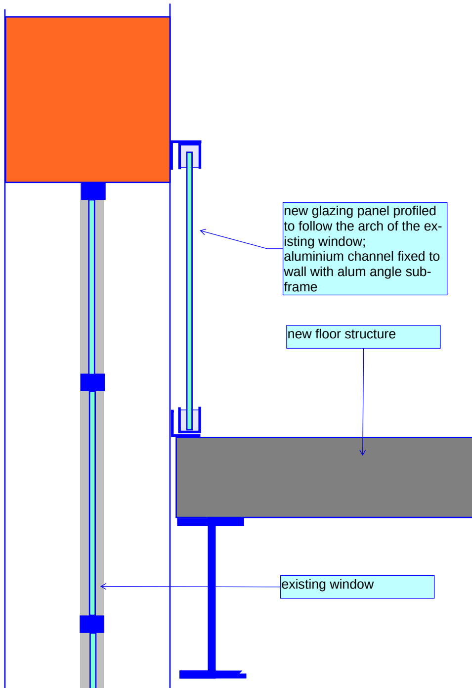
West elevation windows - new floor - junction detail (3 instances)
