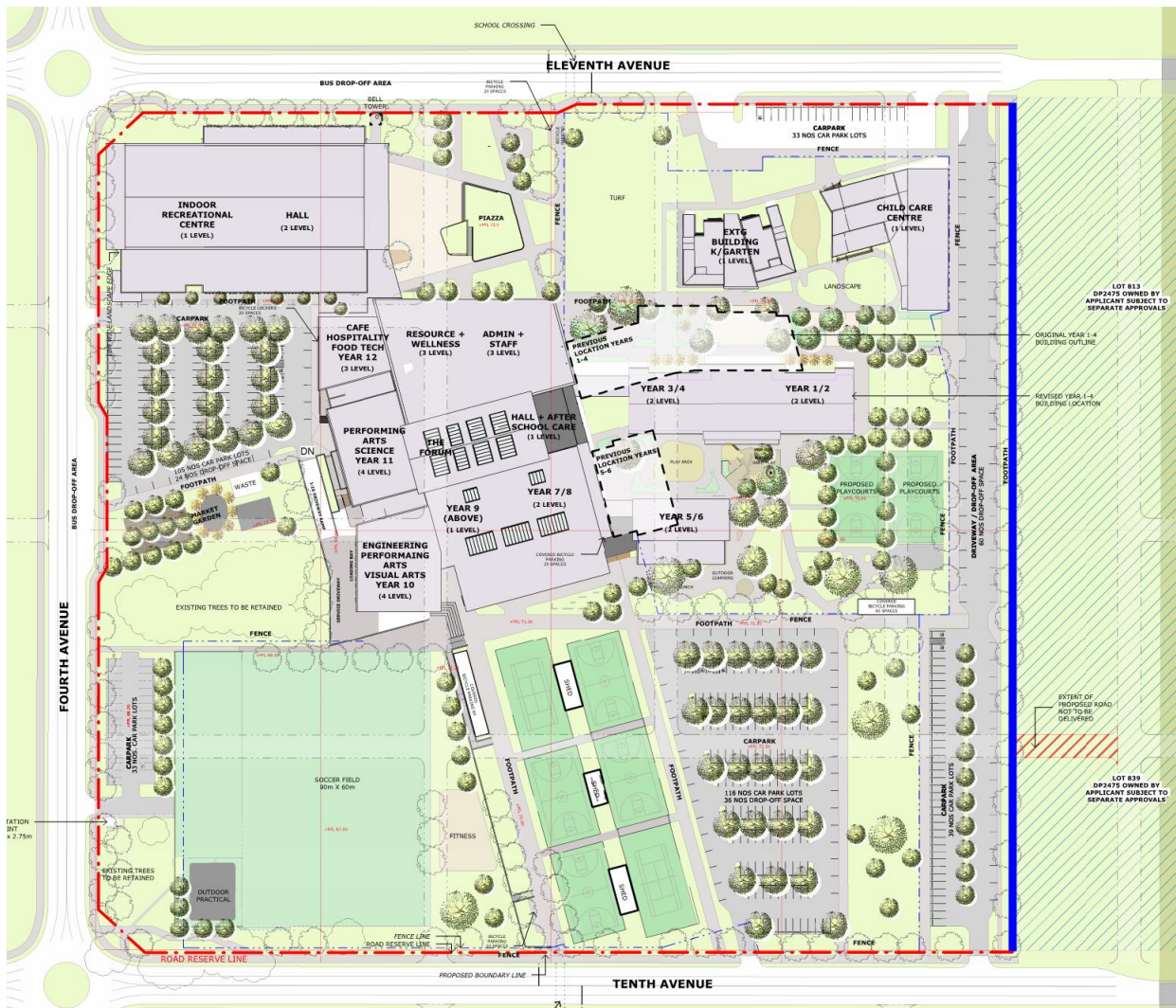
Figure 6: Extent and location of the proposed noise barrier (solid blue line).
