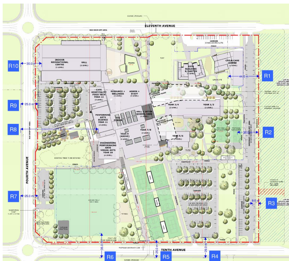
Figure 2: Site layout of the proposed development and distances to nearest noise sensitive receivers.
