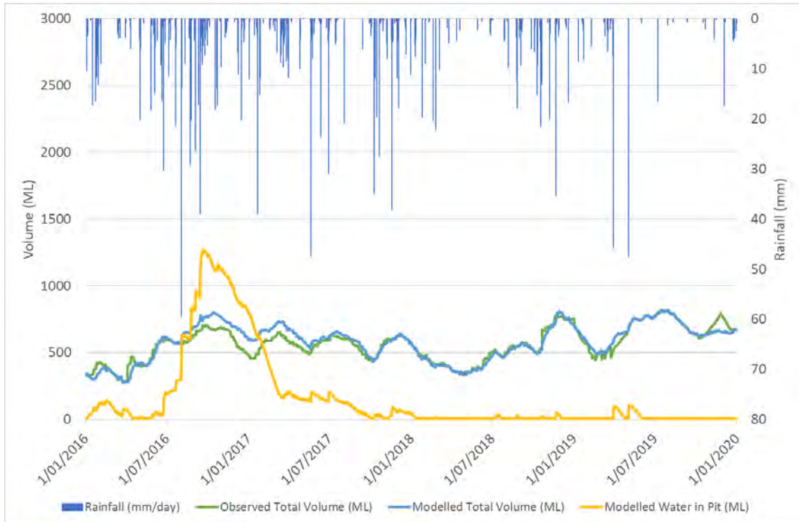
Figure 5-1 Total site water inventory
