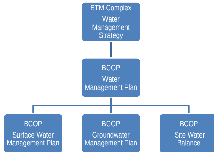
Figure 1-1 Document hierarchy
