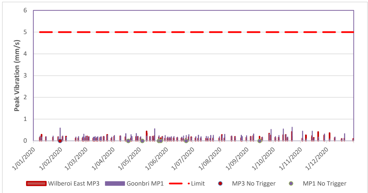
Figure 6-10 Summary of Peak Vibration Monitoring Results
