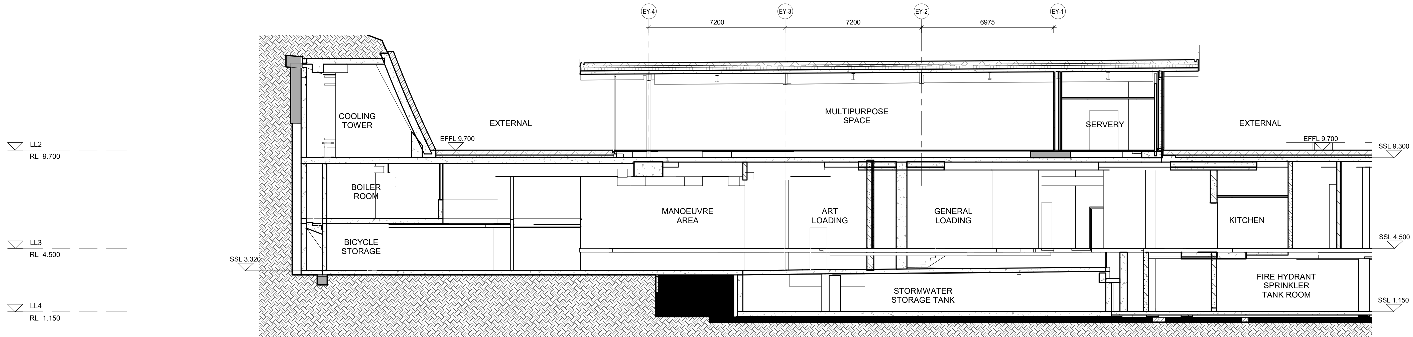
4 Building Section - Zone E - North-South Scale: 1 : 100
