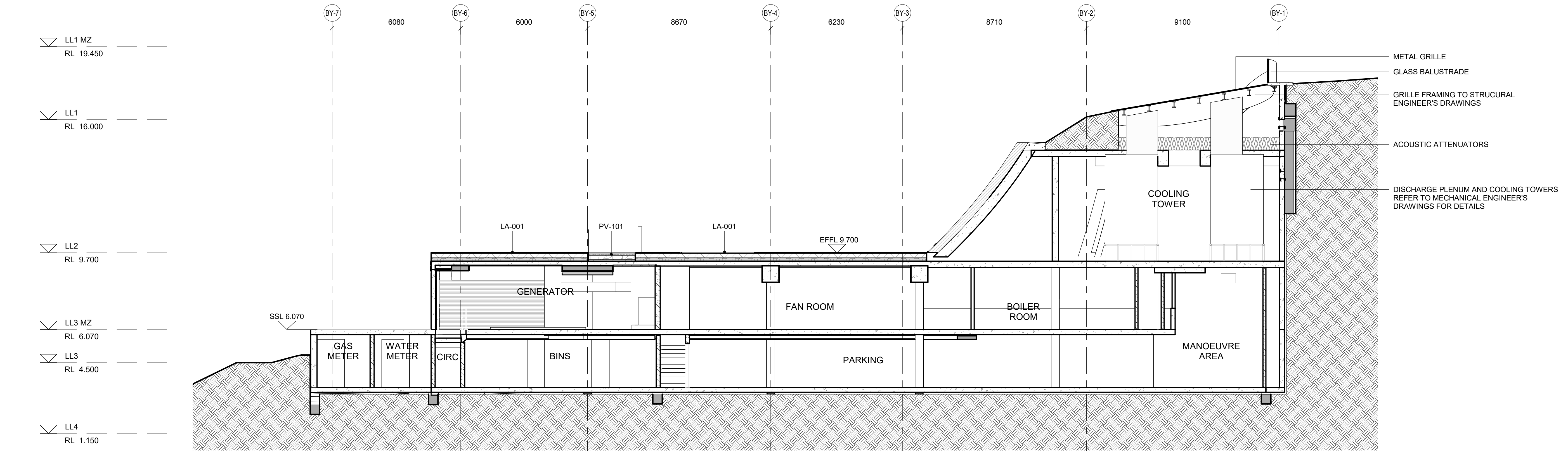
3 Building Section - Zone B - East-West 1 DA Scale: 1 : 100
