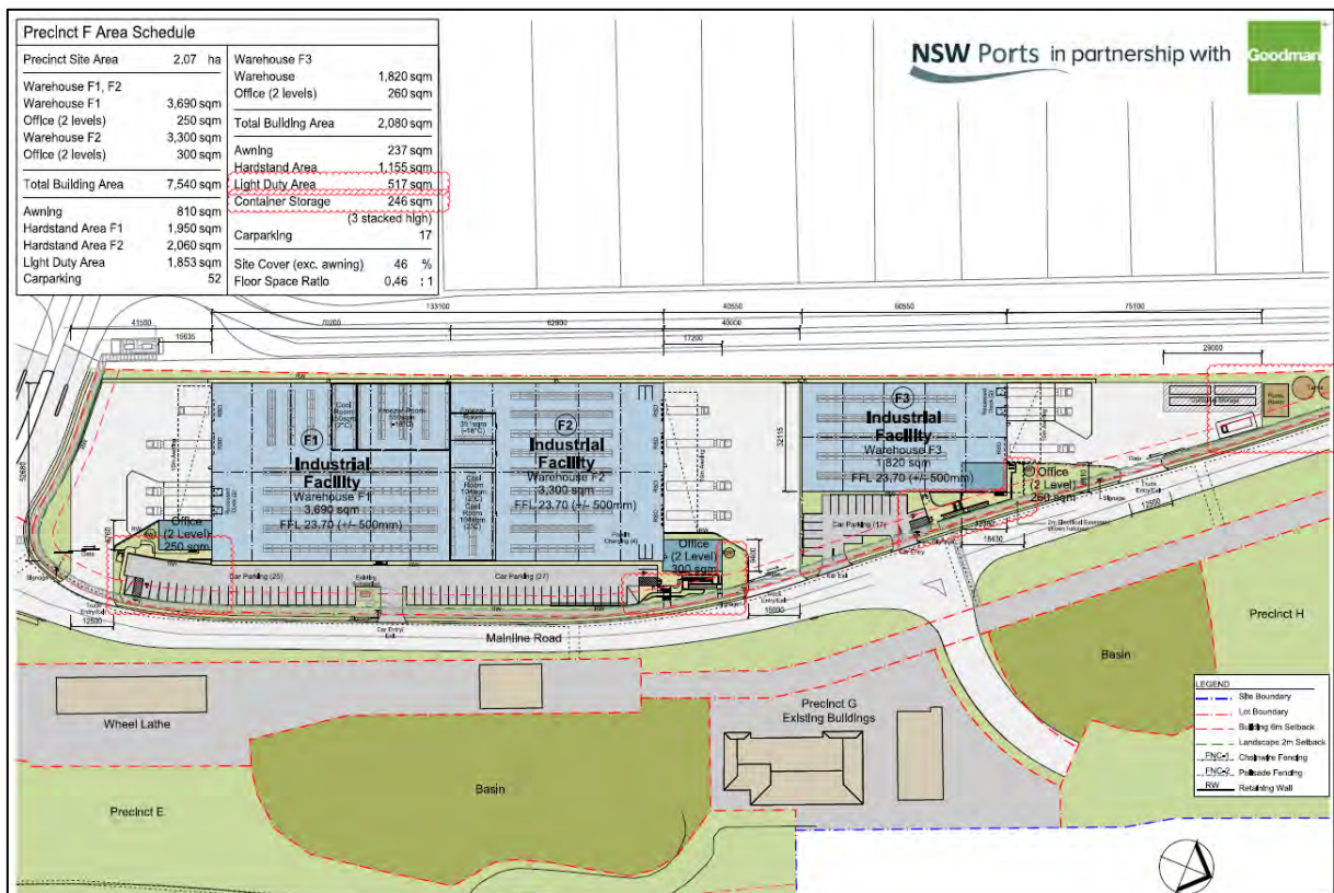
Figure 5: Development Site Plan
