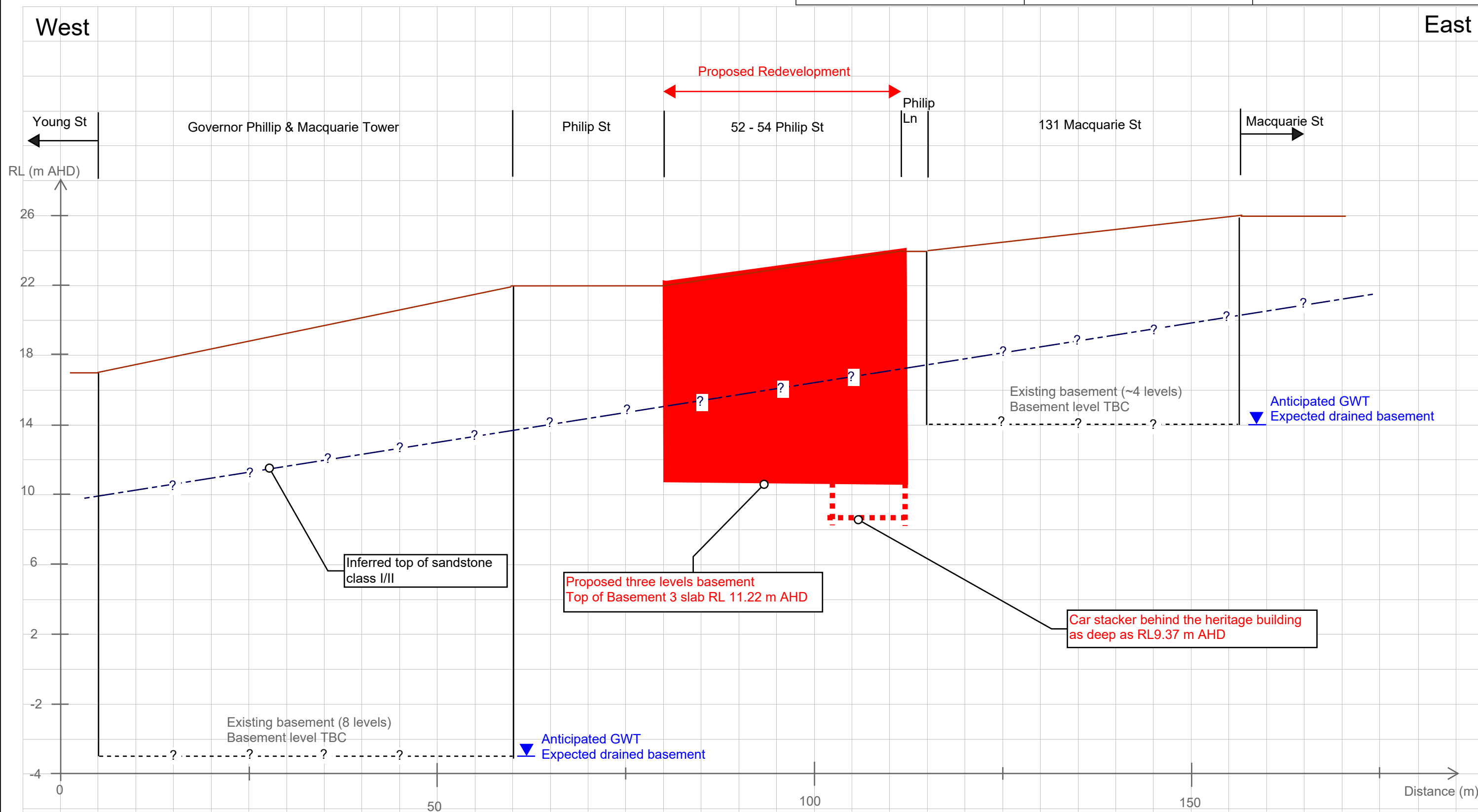
East-West Cross-Section Horizontal scale exaggerated by 2.5
