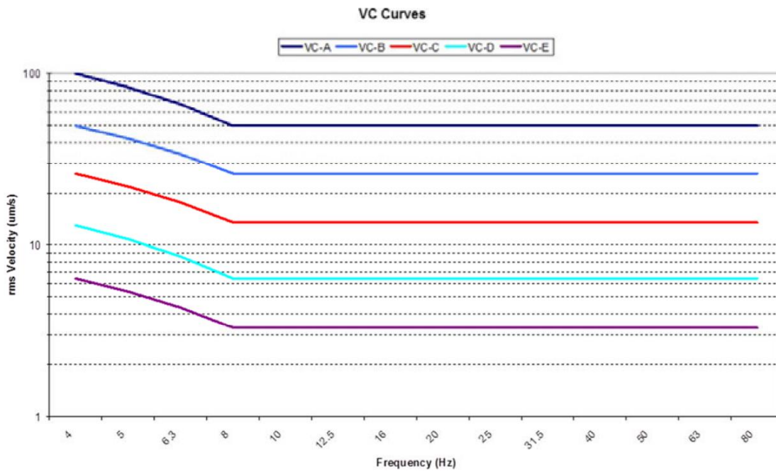
Figure 6-3: Generic Vibration Criterion (VC) curves
