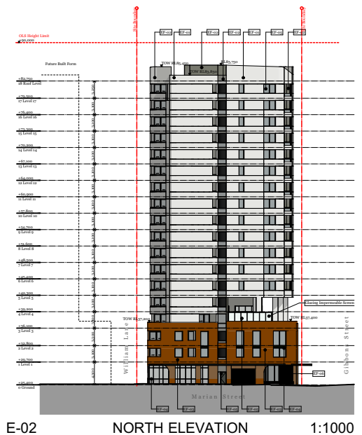
E-02 NORTH ELEVATION 1:1000
