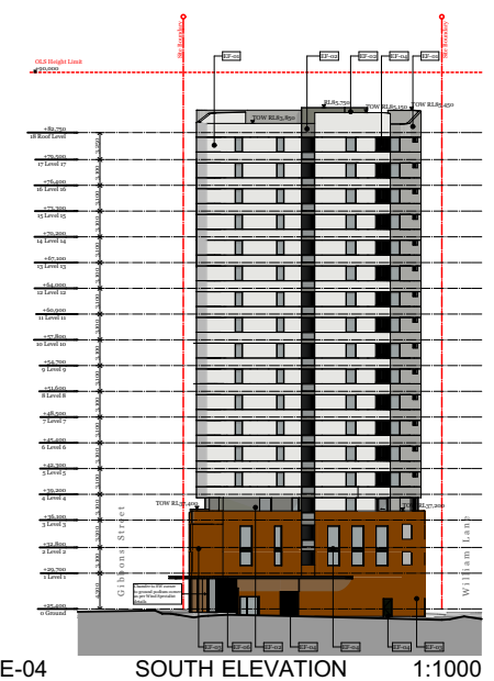
E-04 SOUTH ELEVATION 1:1000
