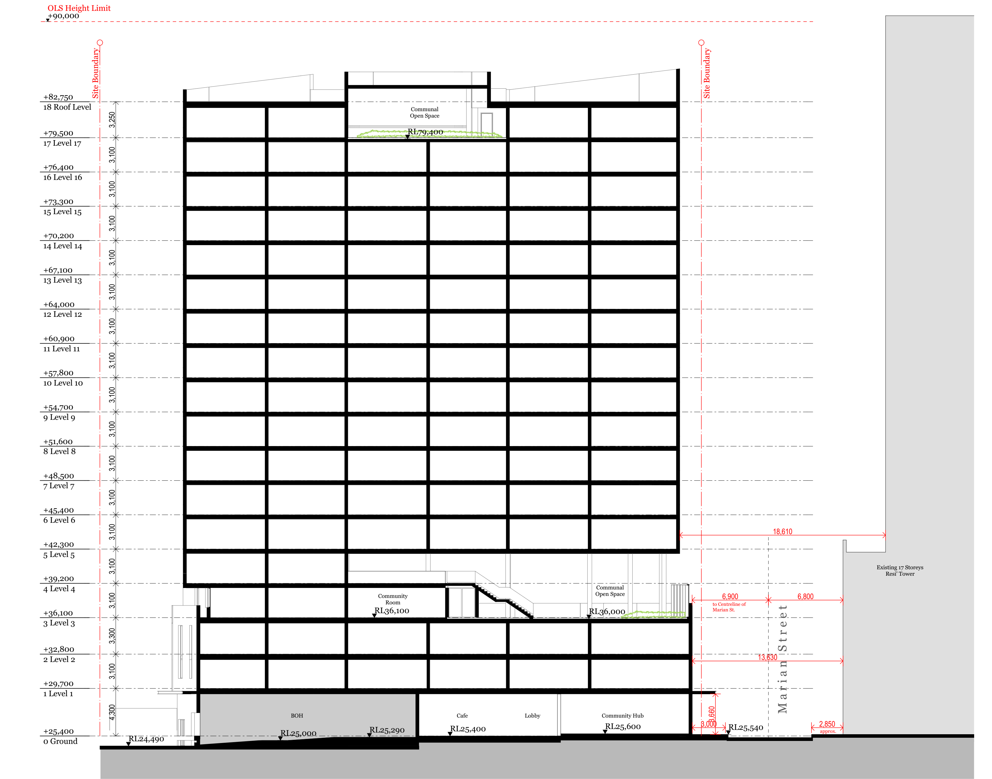
S04 Section 4 1:200
