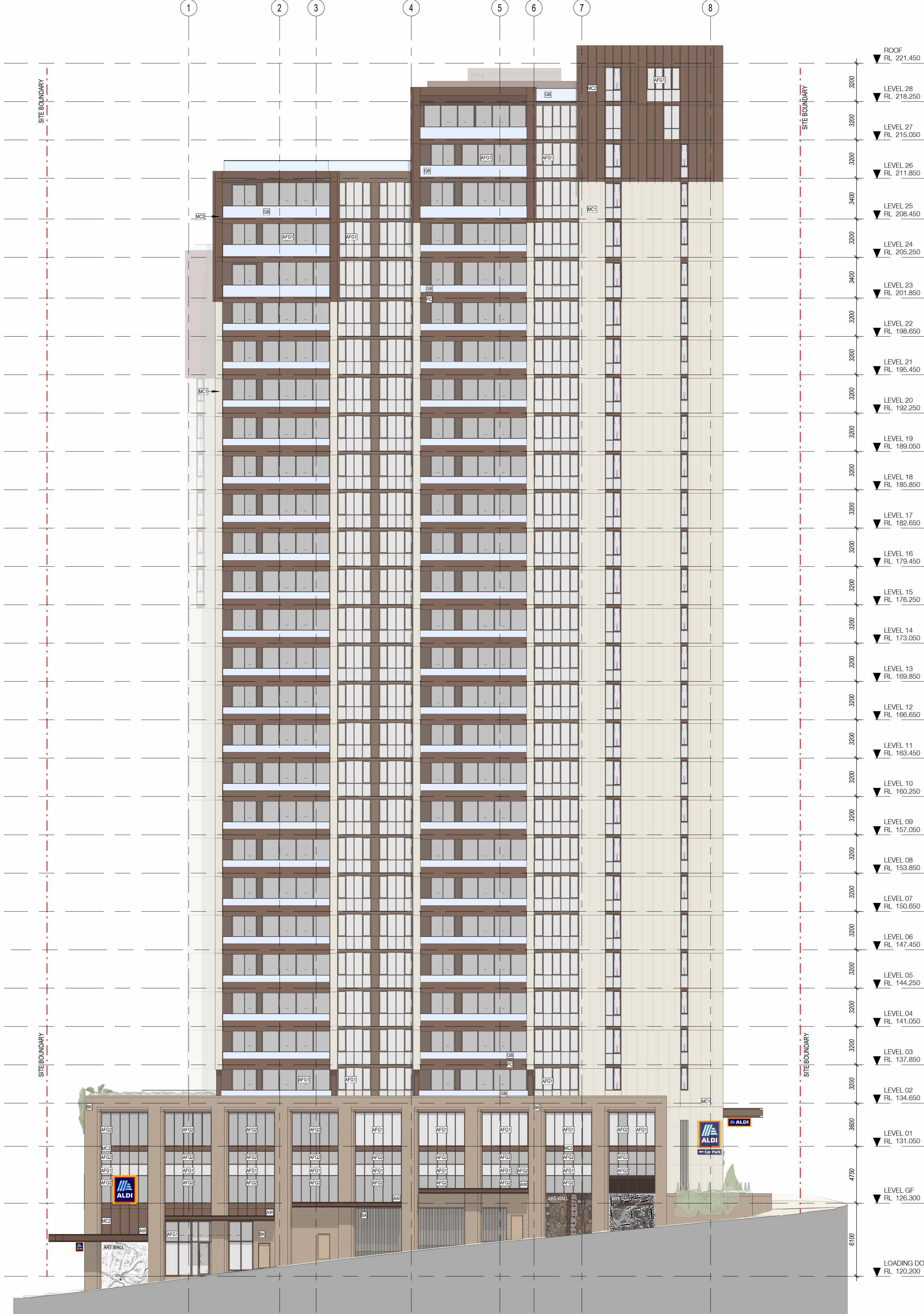
1 ELEVATION SOUTH 1 : 200
