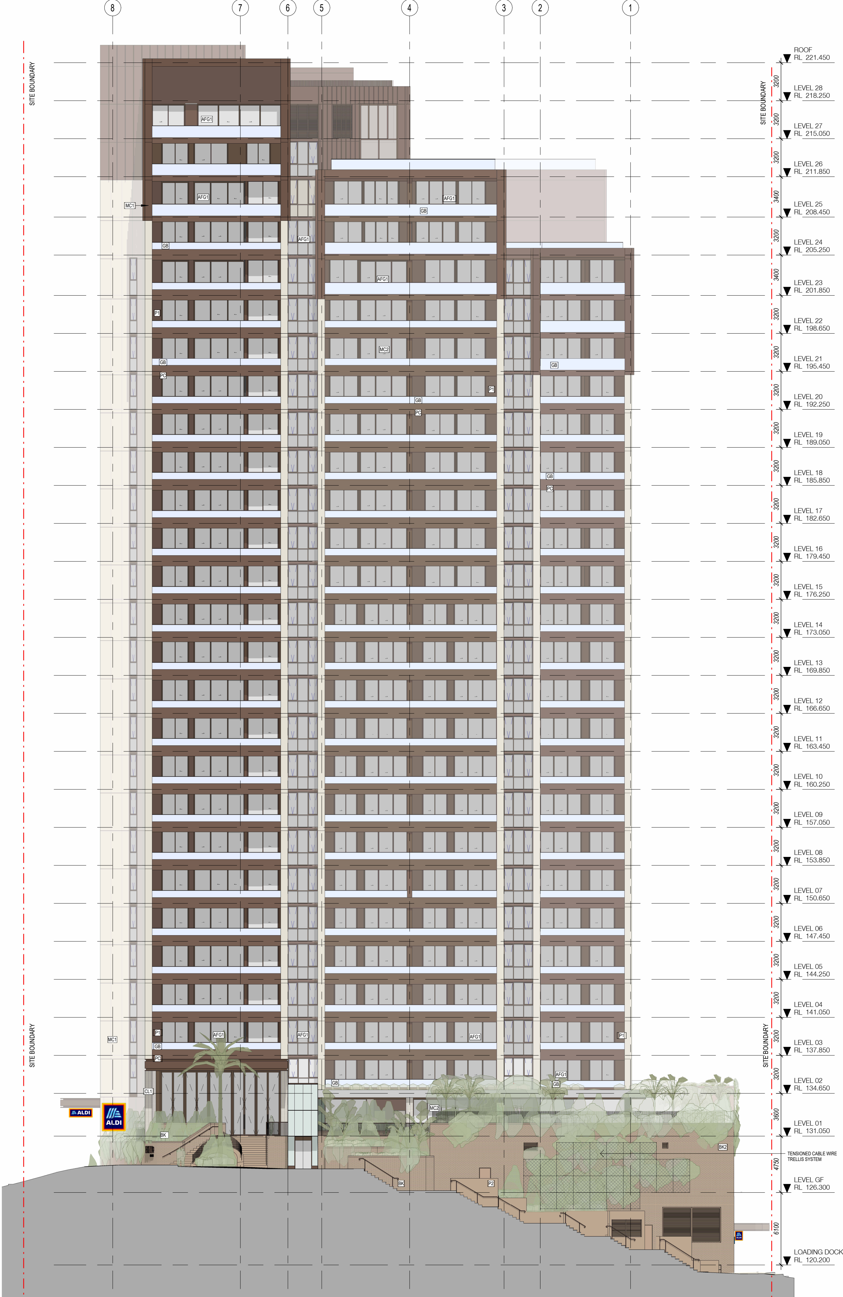
1 ELEVATION - NORTH 1 : 200
