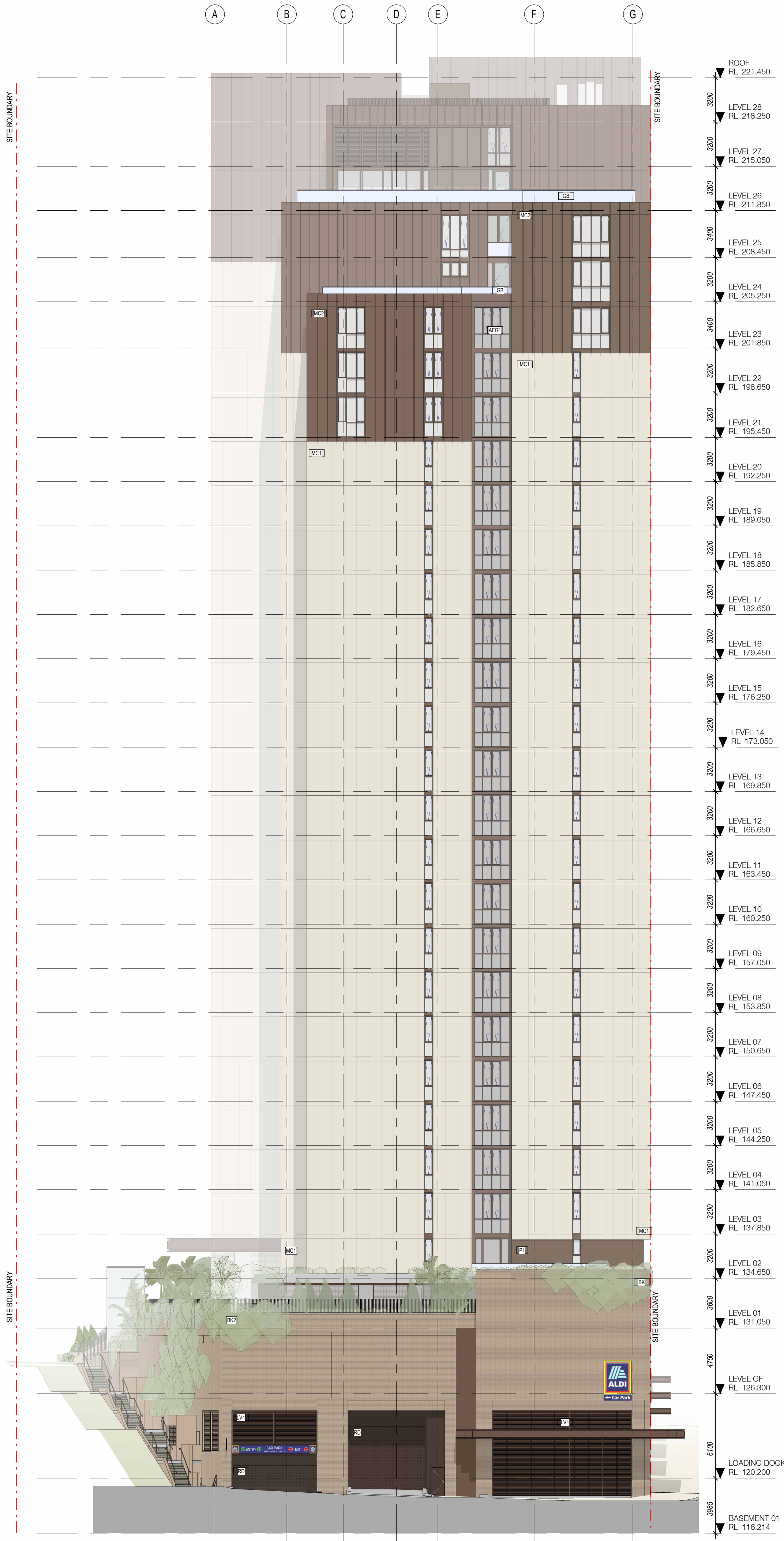
1 ELEVATION - WEST 1 : 200
