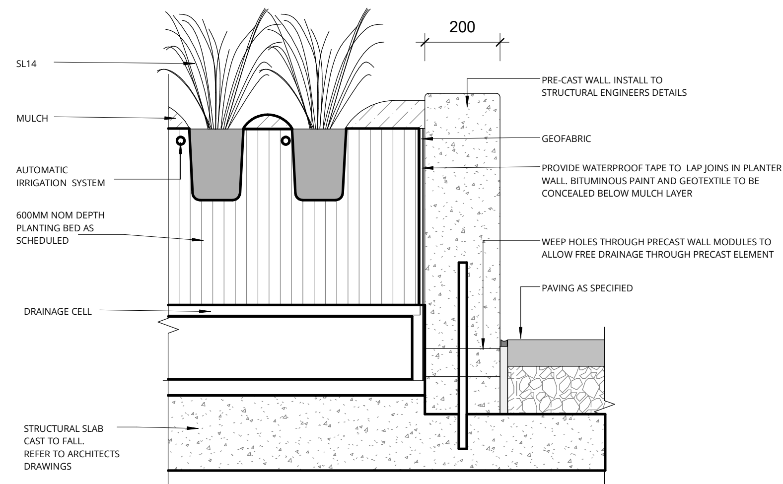
4 PLANTING - INSITU CONCRETE WALL 1 : 10
