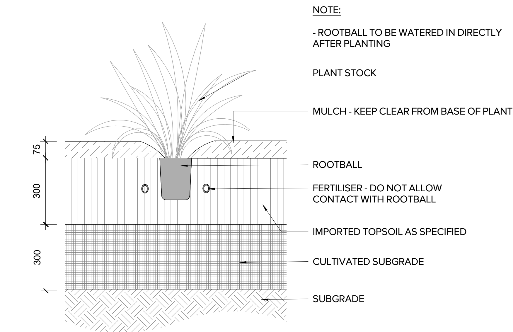
3 PLANTING - SHRUB 1 : 10
