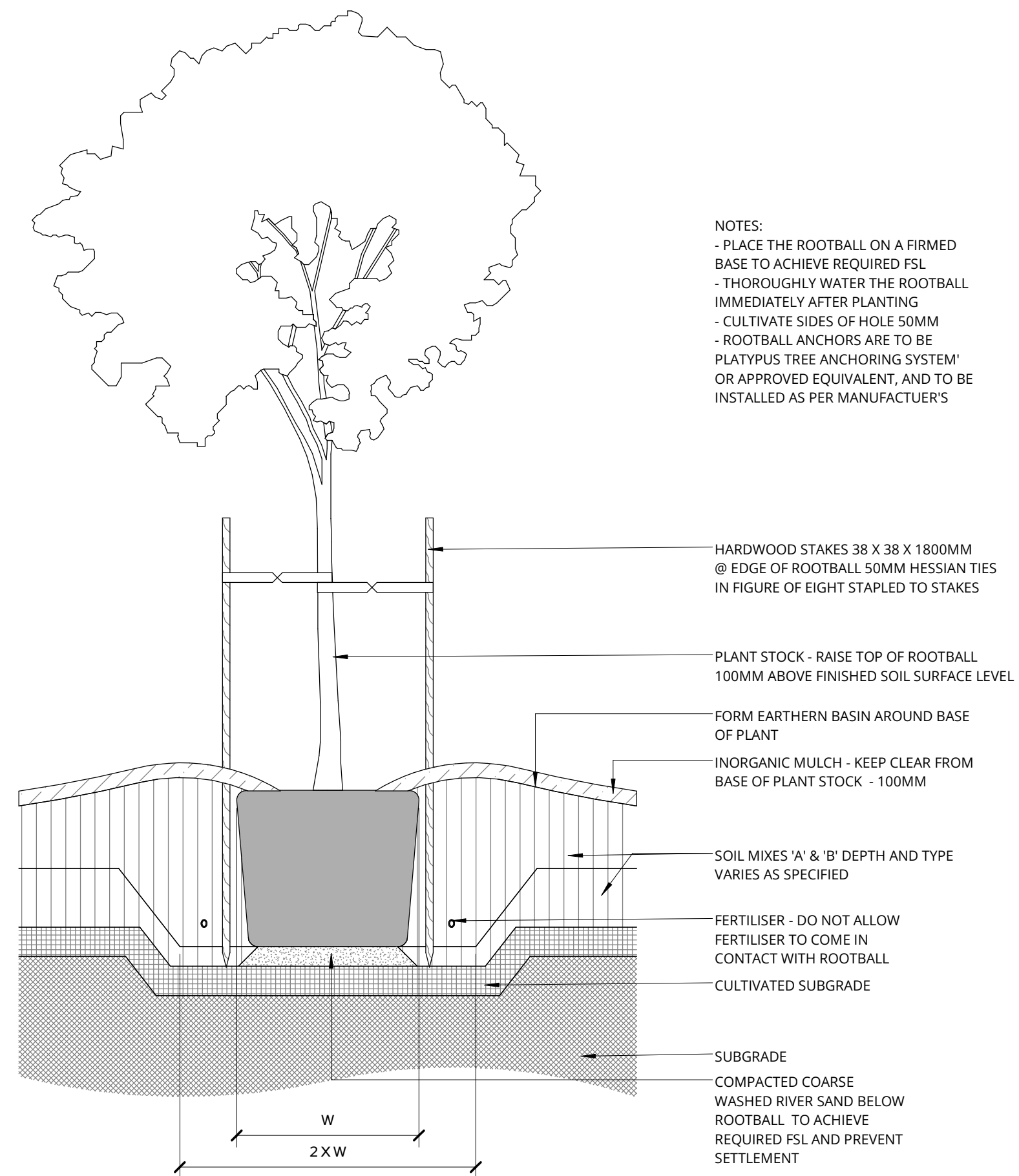
5 TREE - 400-1000L - TIMBER STAKES 1 : 25
