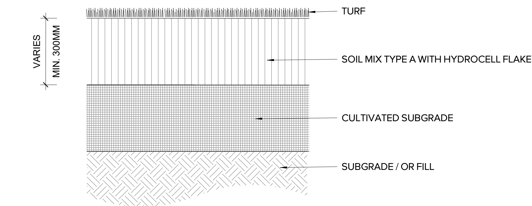
1 TURF - ON GRADE 1 : 10
