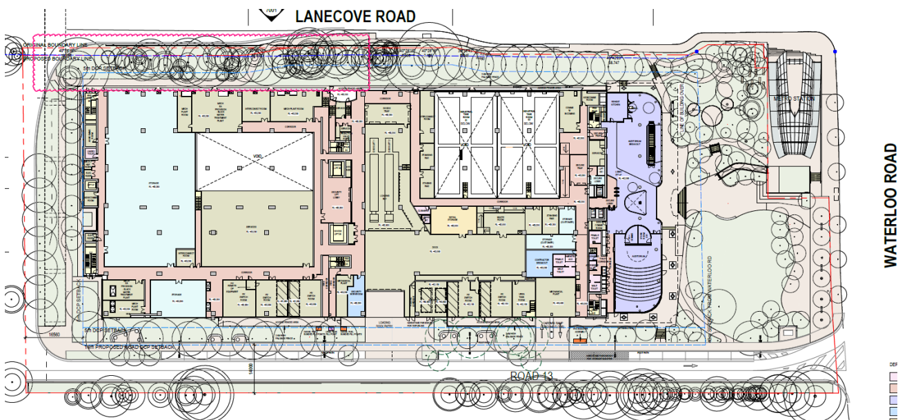
Figure 3 – Proposed Level 01 Floor Plan. Source: HDR – February 2026
