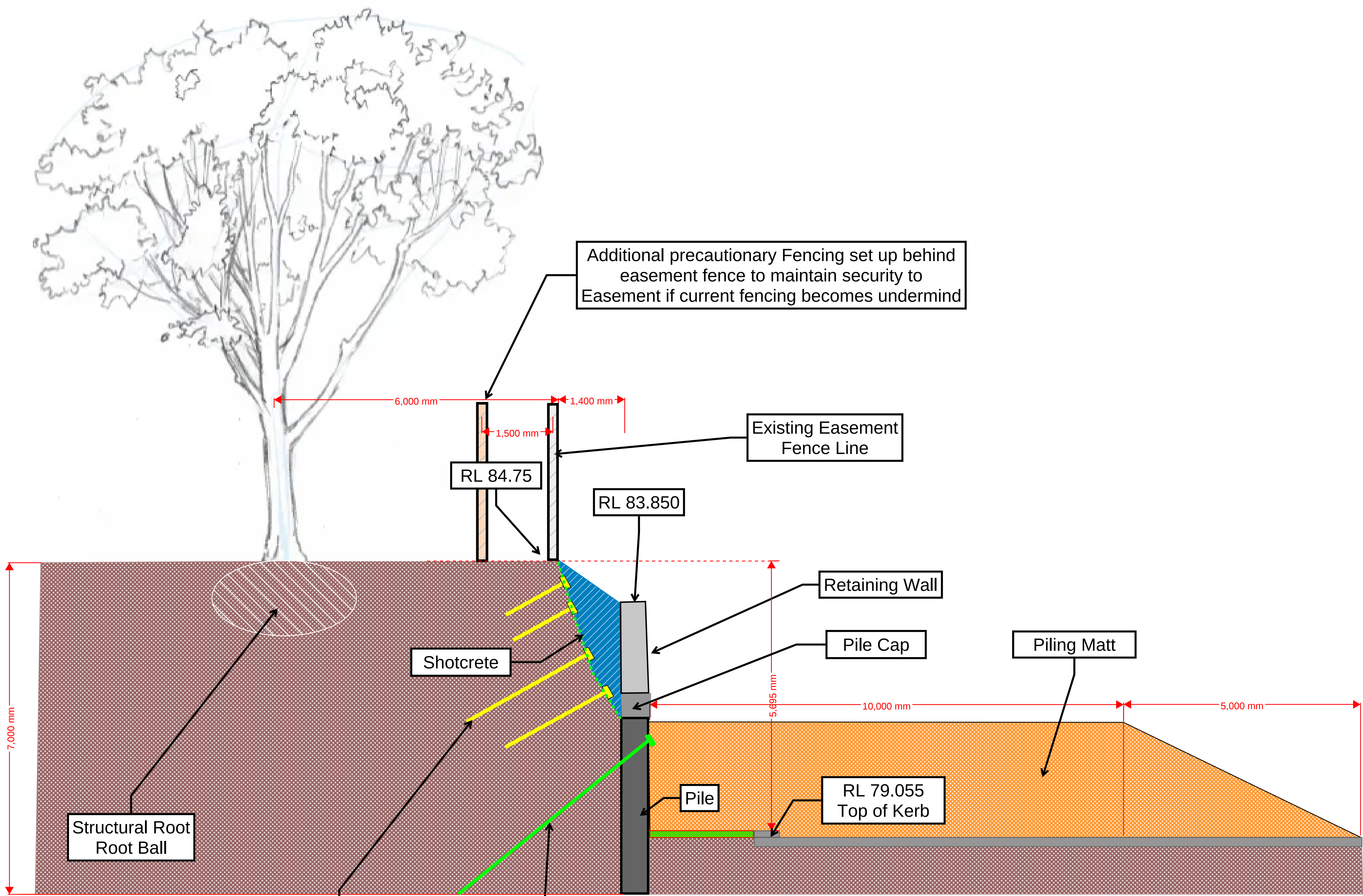
Section C-C
