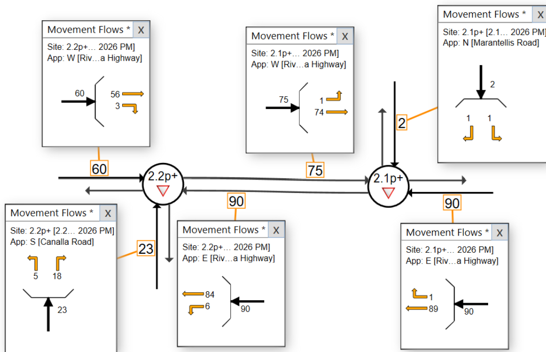
Figure 23 - SIDRA Model 2026 PM (Development Construction) – Movement flows
