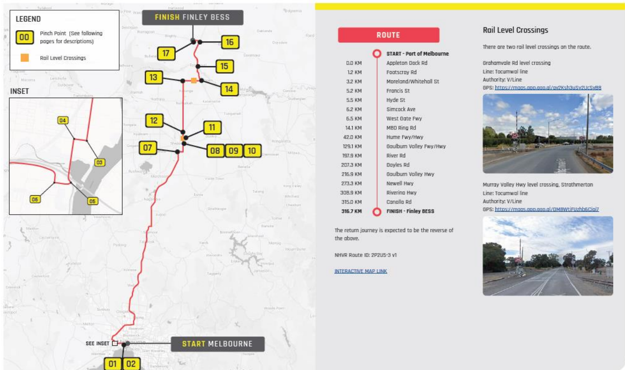
Figure 5 - Proposed OSOM route for transformer transportation (source: OSOM Route Survey, Ares Group, January 2026)
