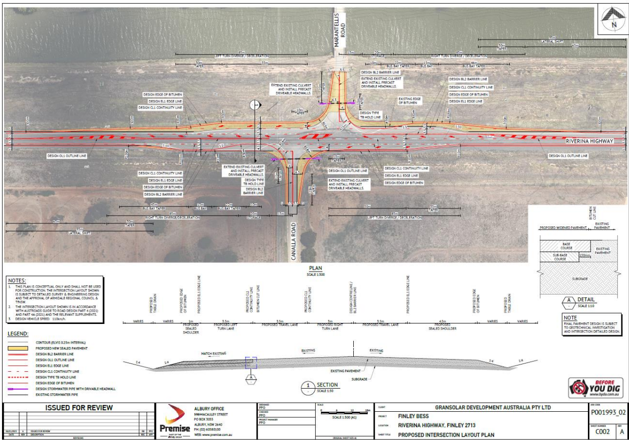
Figure 28 - Alternative configuration for Riverina Highway, Canalla Road, Marantellis Road intersection - CHR/AUL
