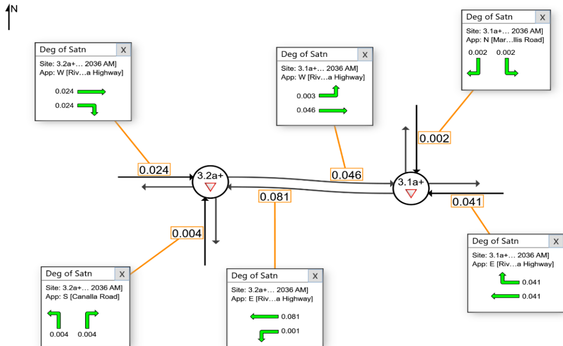
Figure 25 - SIDRA Model 2036 AM (Post Development) – DoS
