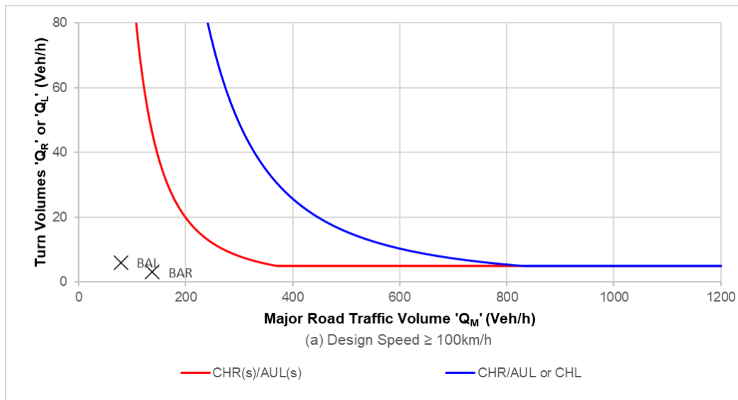
Figure 19 Major Road Turn Warrants – Right and Left Turn – PM peak
