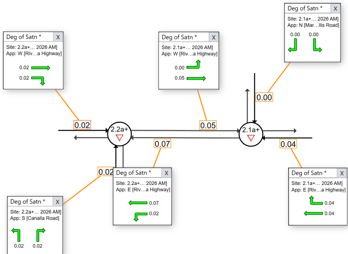
Figure 22 - SIDRA Model 2026 AM (Development Construction) – DoS
