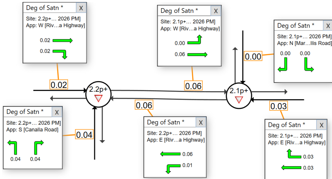
Figure 24 - SIDRA Model 2026 PM (Development Construction) – DoS
