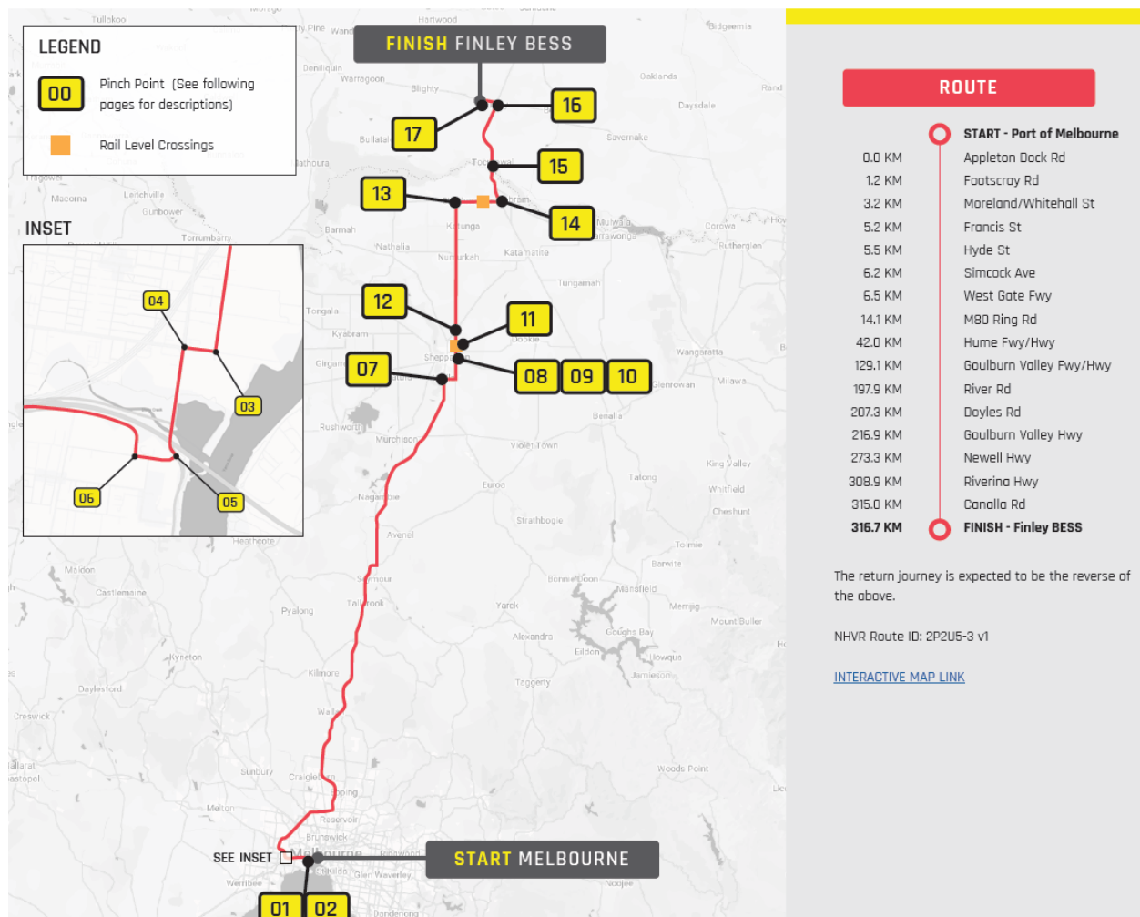
Figure 29 - Proposed OSOM route for transformer transportation (source: OSOM Route Survey, Ares Group, January 2026)
