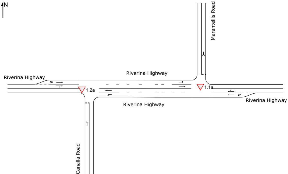
Figure 20 - SIDRA Model Geometry
