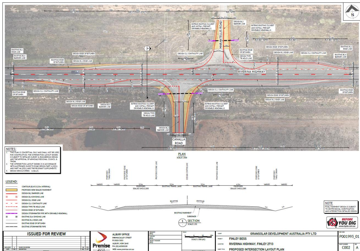
Figure 27 - Proposed upgrade of Riverina Highway, Canalla Road and Marantellis Road intersection - BAL/BAR configuration
