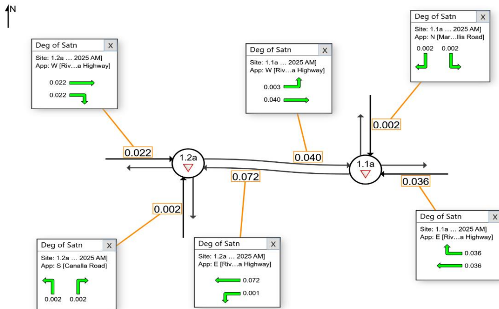
Figure 6 - SIDRA Model 2025 AM (No Development) – DoS
