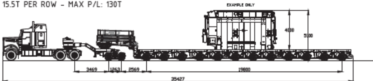
Figure 4 - The largest vehicle anticipated to access the site (source: OSOM Route Study, Ares Group, Jan 2026)
