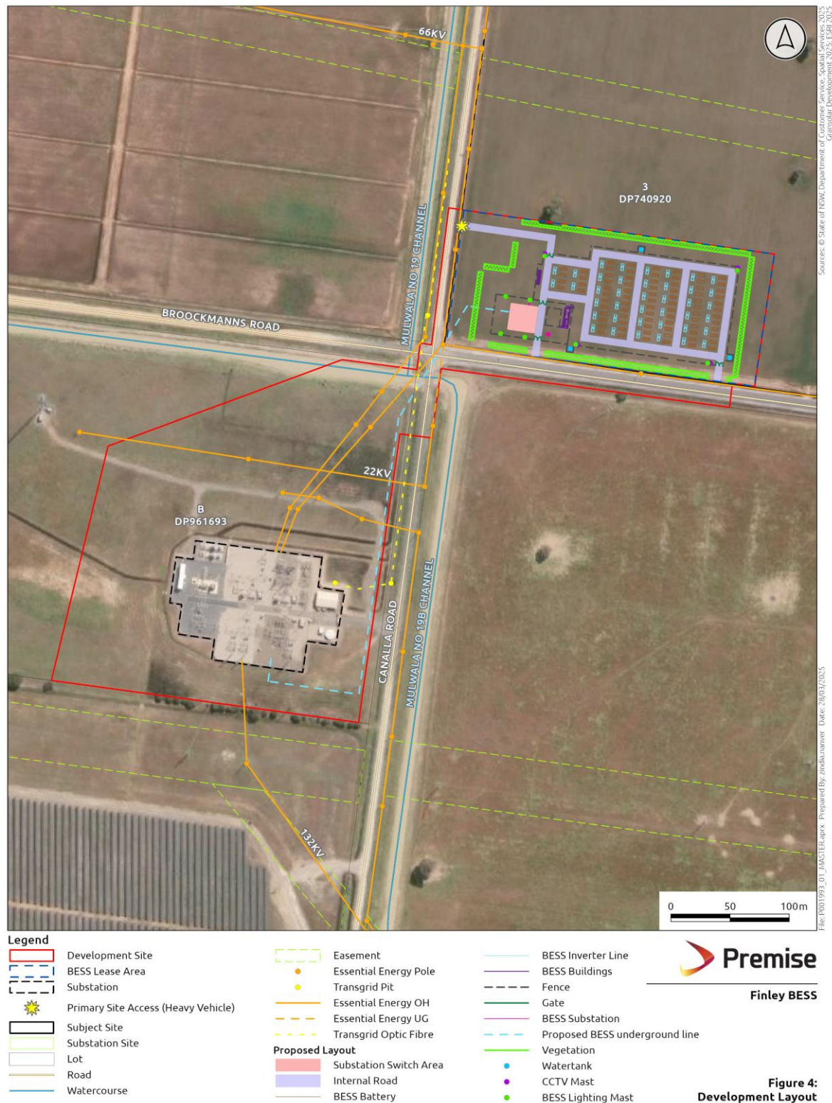
Figure 3-2: Development Site Layout
