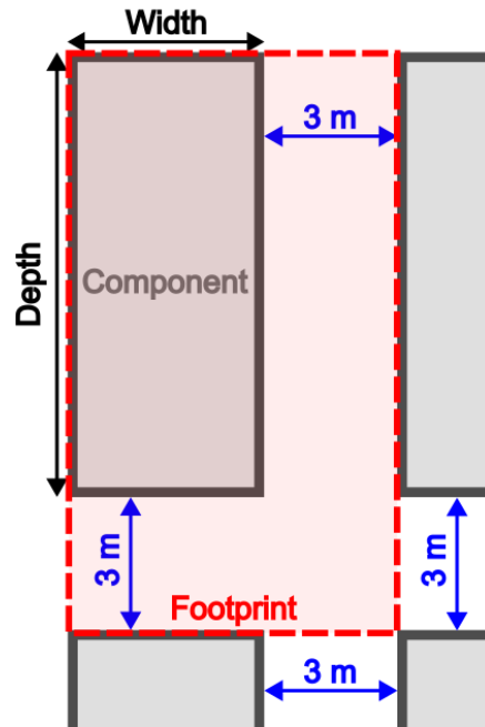
Figure 4-3: Illustration of BESS Unit Footprint Tiling, Considering Separation Distance
