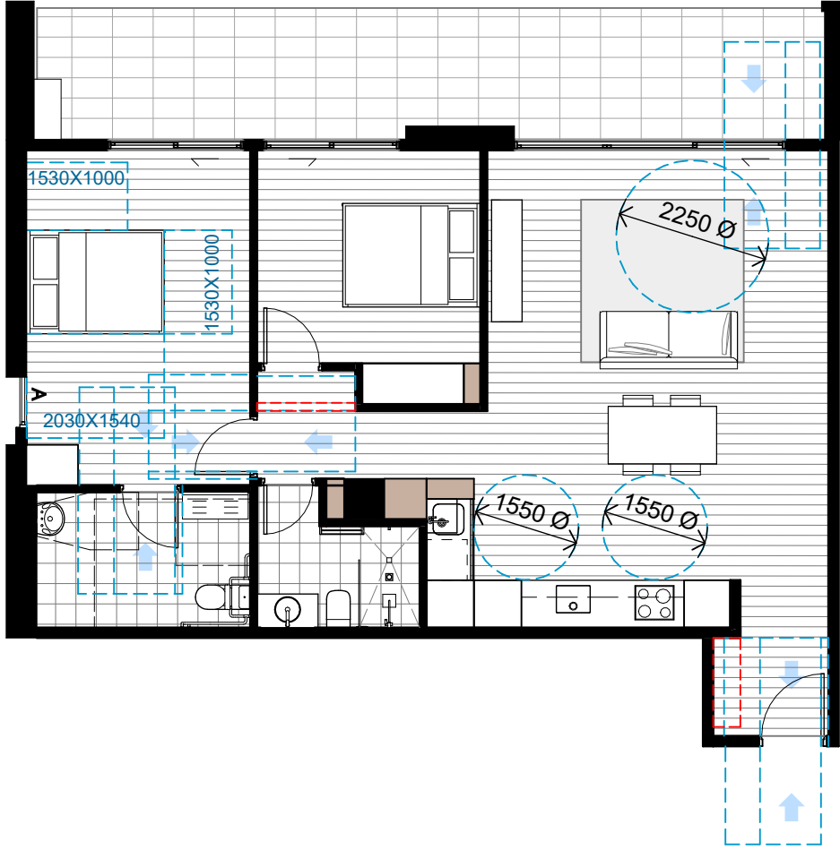
3 2B_4_02_VM Post Adaptable SCALE 1 : 100
