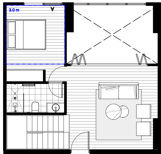
3 3B_6_03_VM Lower SCALE 1 : 100
