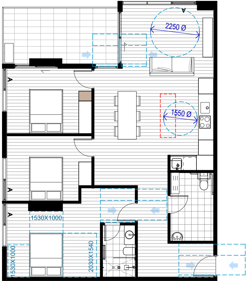
2 3B_6_05_VM Post Adaptable SCALE 1 : 100
