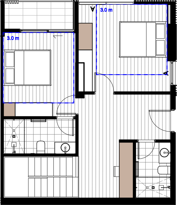
7 2B_7_06_VM Lower SCALE 1 : 100
