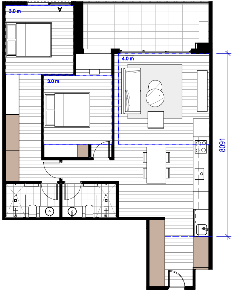
1 2B_5_01_VM SCALE 1 : 100
