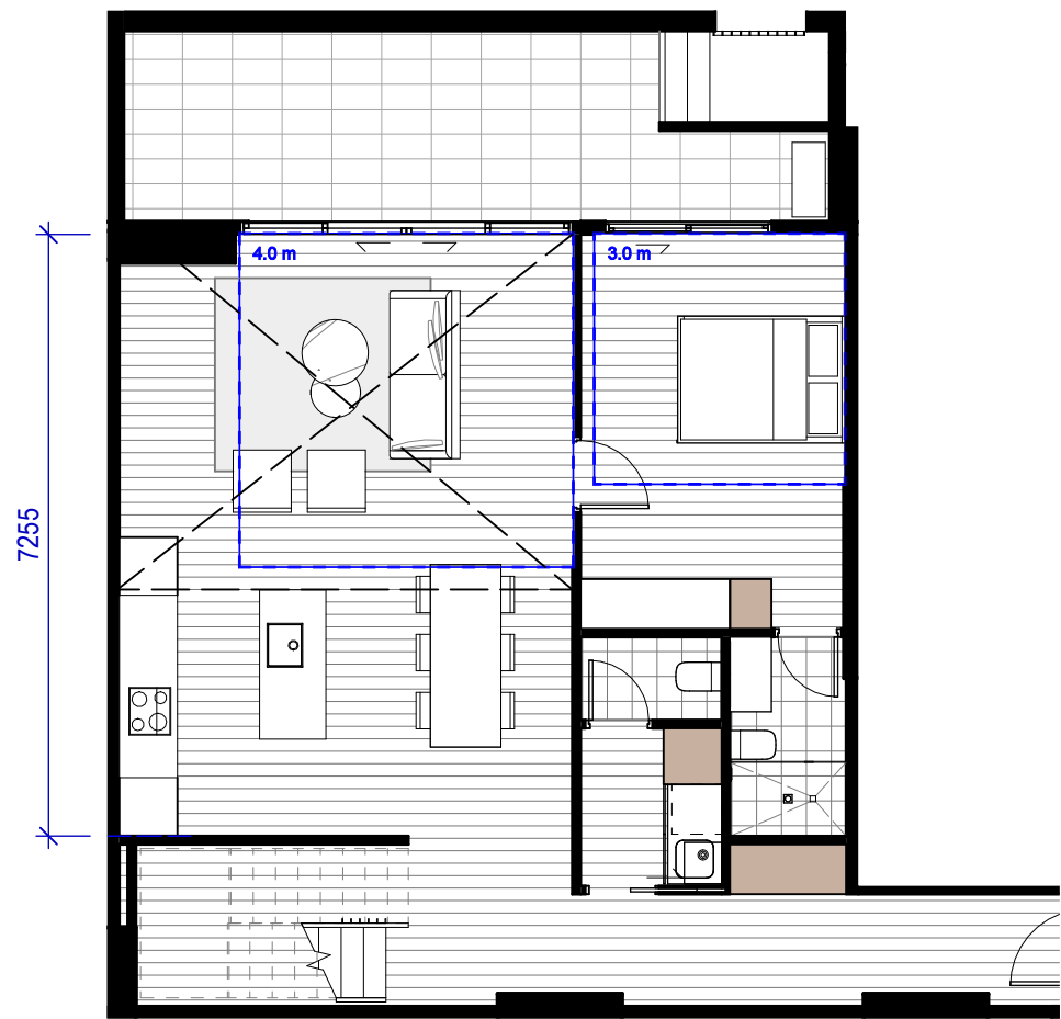
1 3B_6_01_VM Lower SCALE 1 : 100
