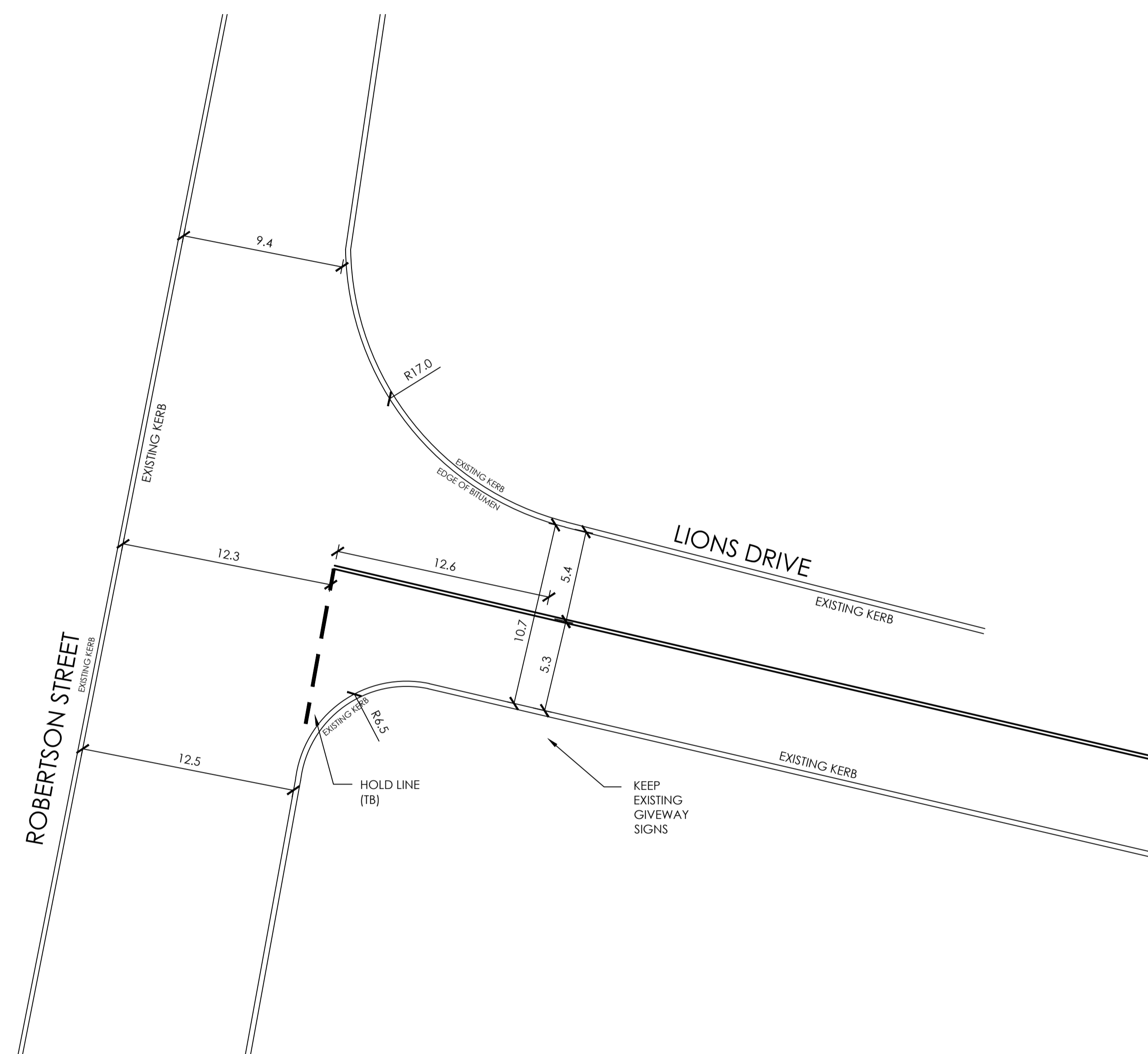
ROBERTSON STREET AND LIONS DRIVE SCALE 1:200 AT A1
