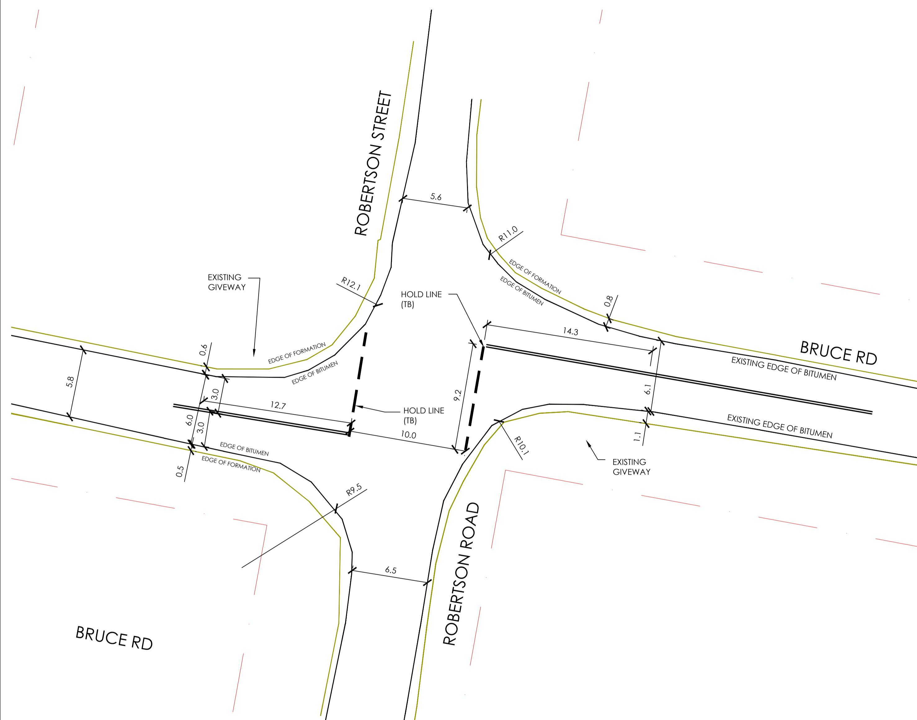
ROBERTSON STREET AND BRUCE ROAD SCALE 1:200 AT A1
