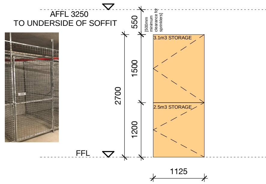
Elevation - Configuration B
