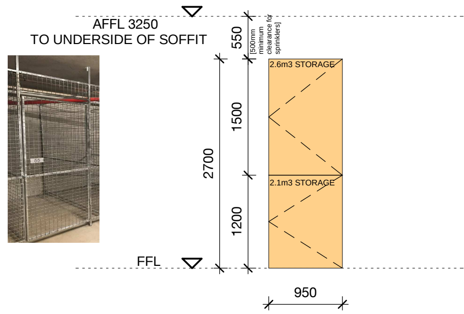
Elevation - Configuration B
