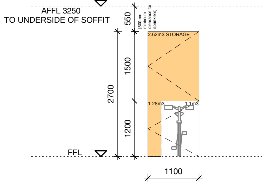
Elevation - Configuration A
