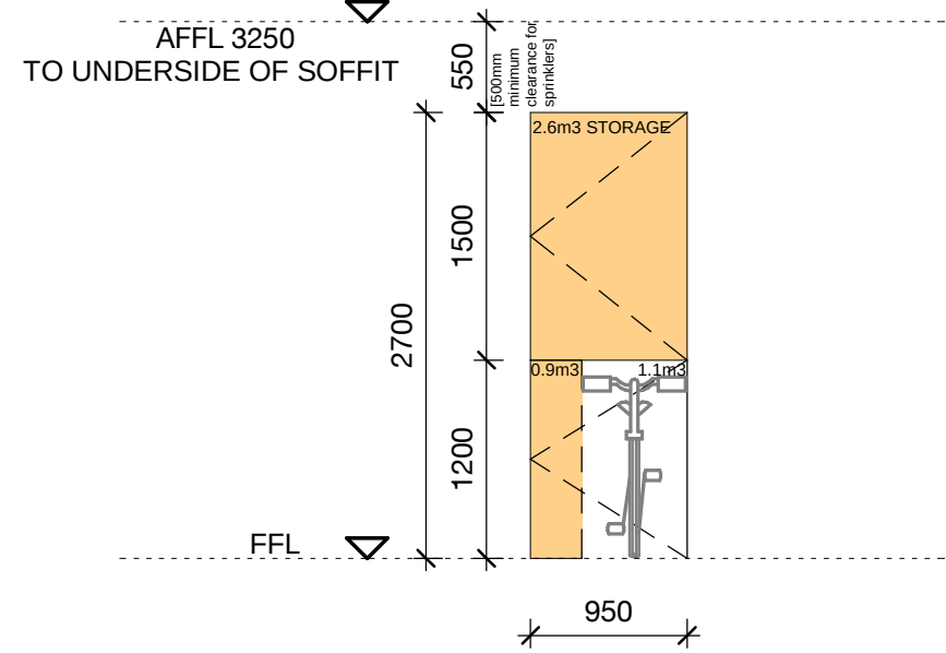
Elevation - Configuration A
