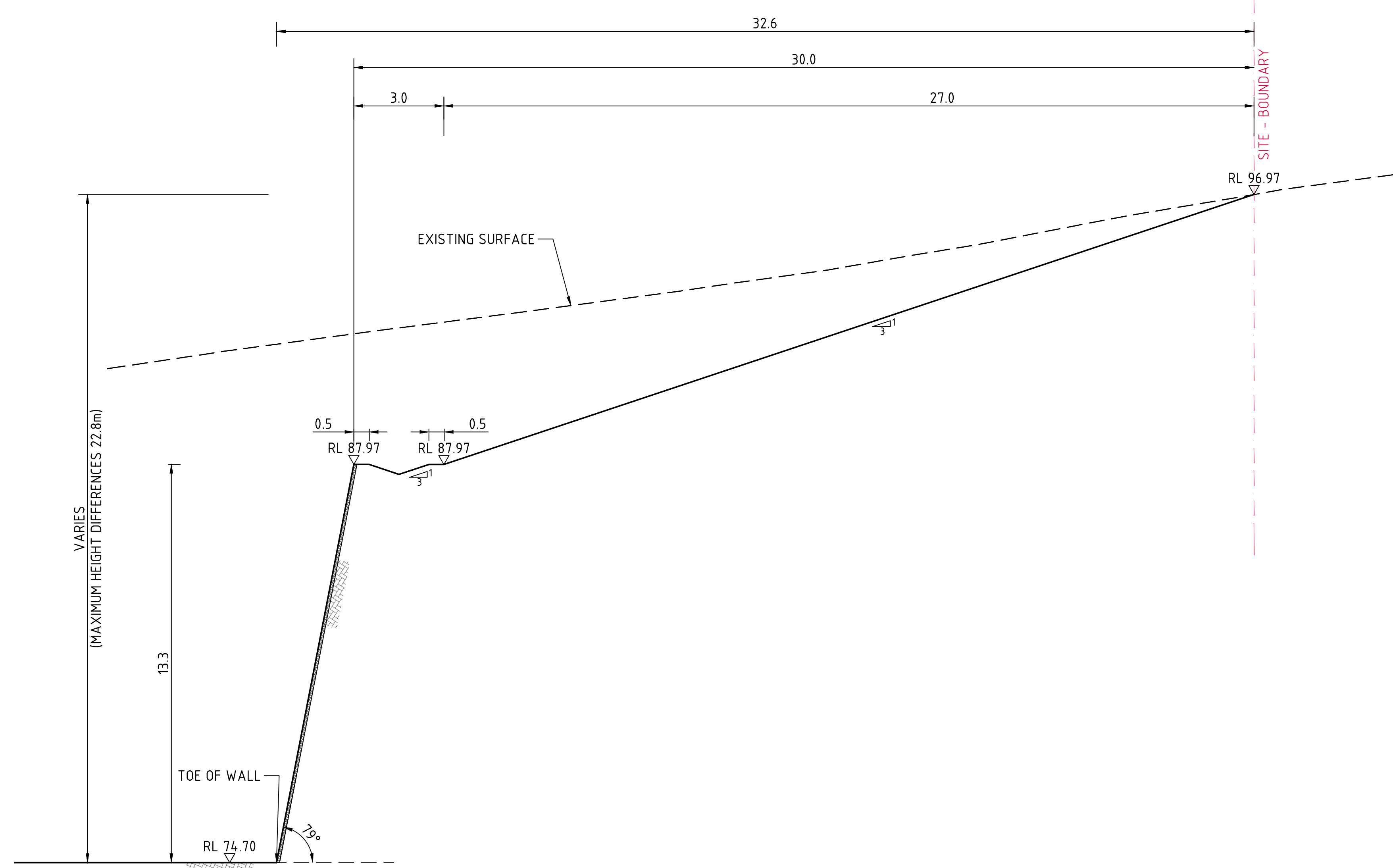
SECTION 1:100 OPTION 1 1/600
