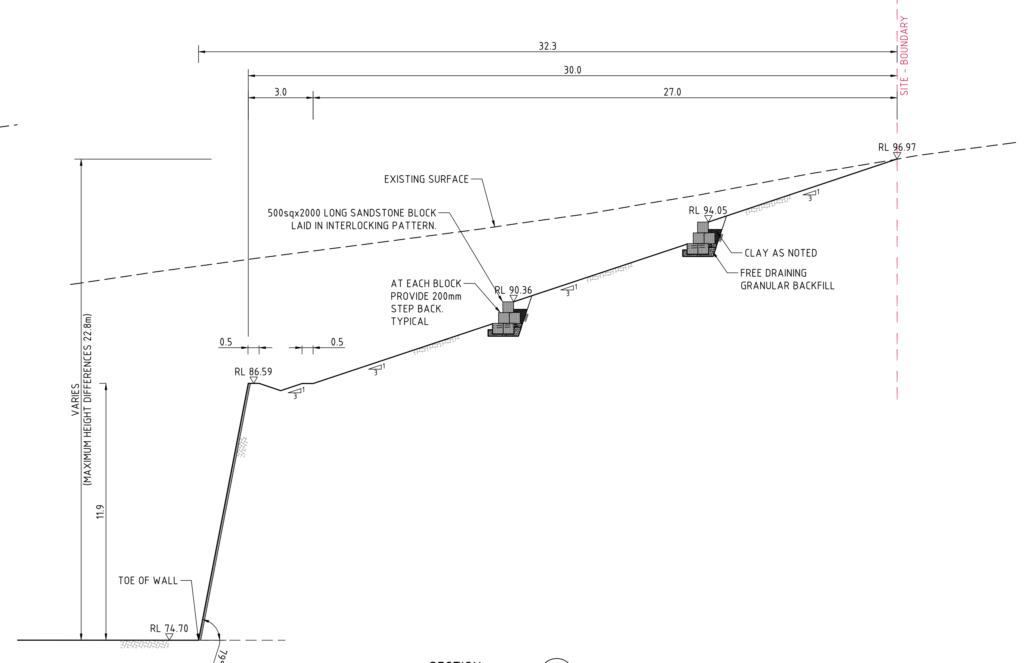
SECTION 1:100 OPTION 2 1/600
