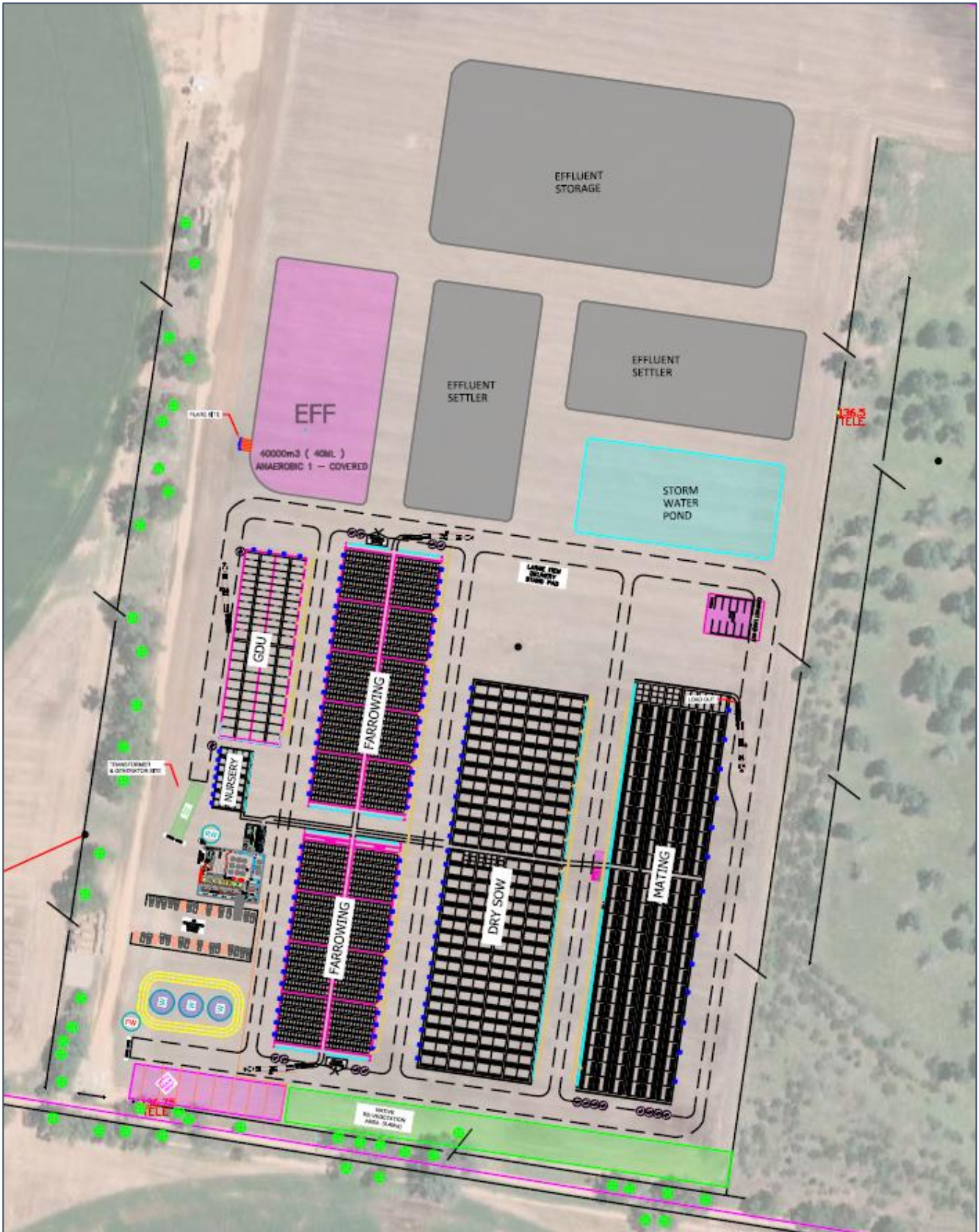
Figure 1: Preliminary Site Layout Plan (JBS, 2025)
