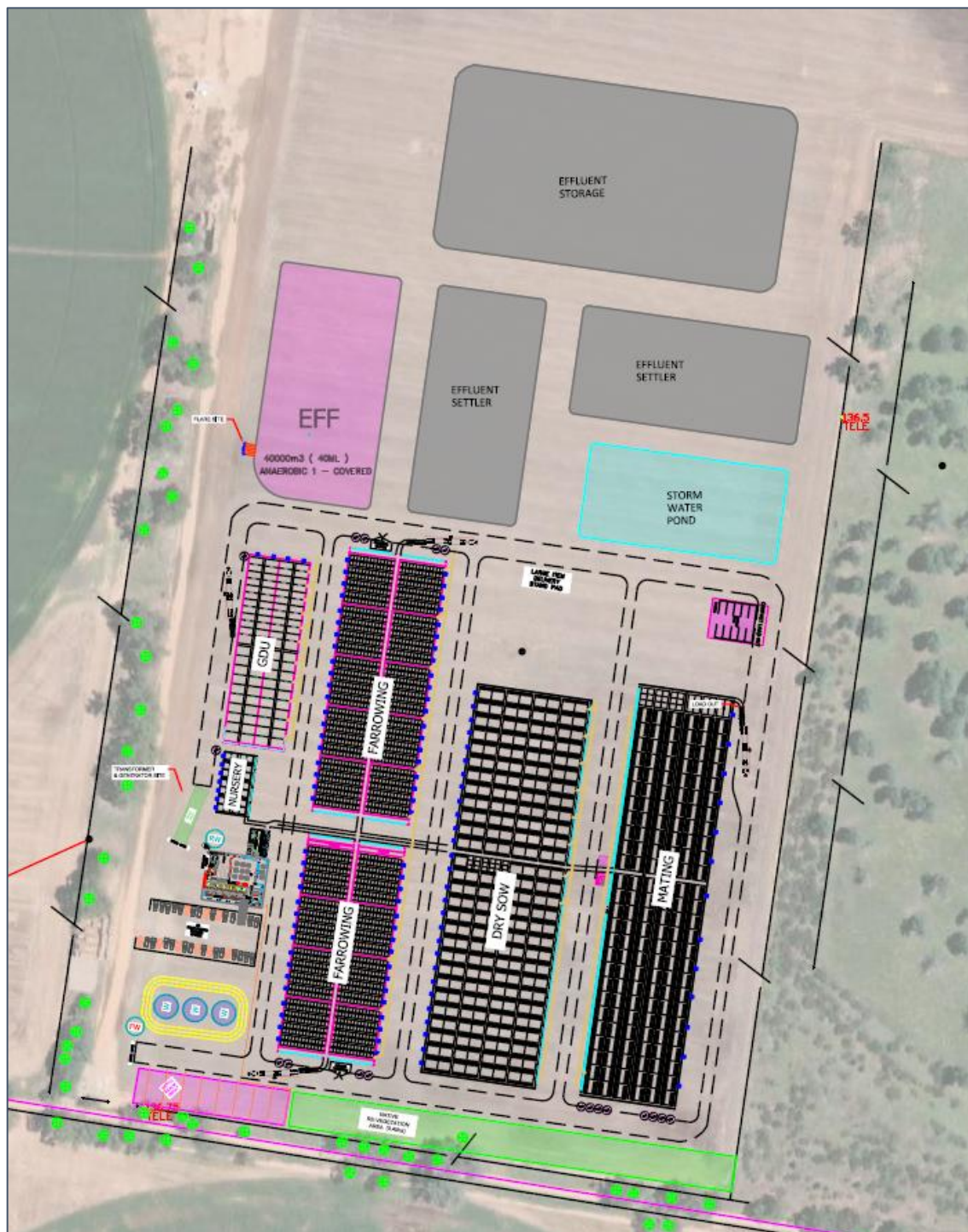
Figure 9: Preliminary Site Layout Plan (JBS, 2025)
