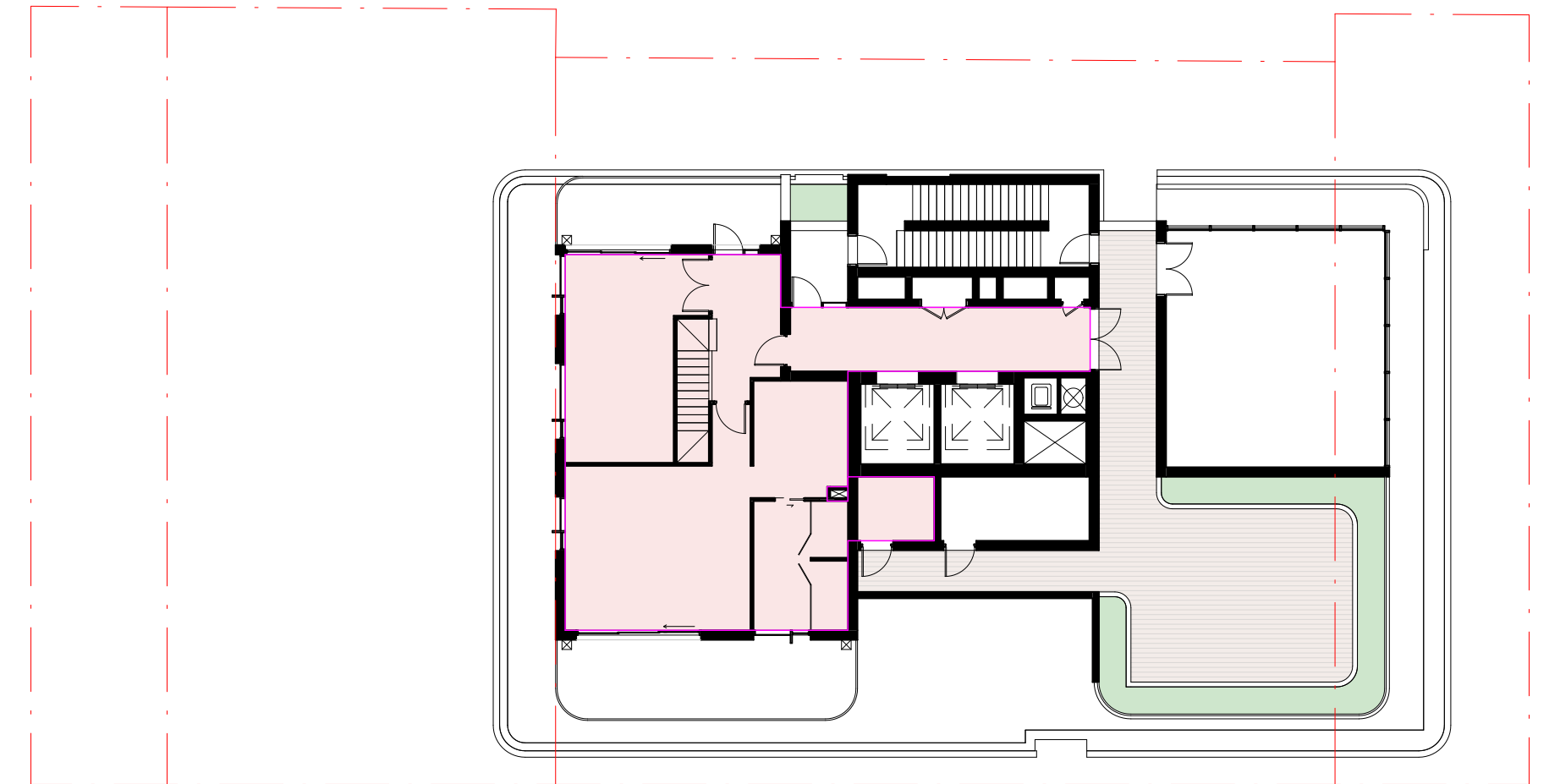
7 LEVEL 13 1:200
