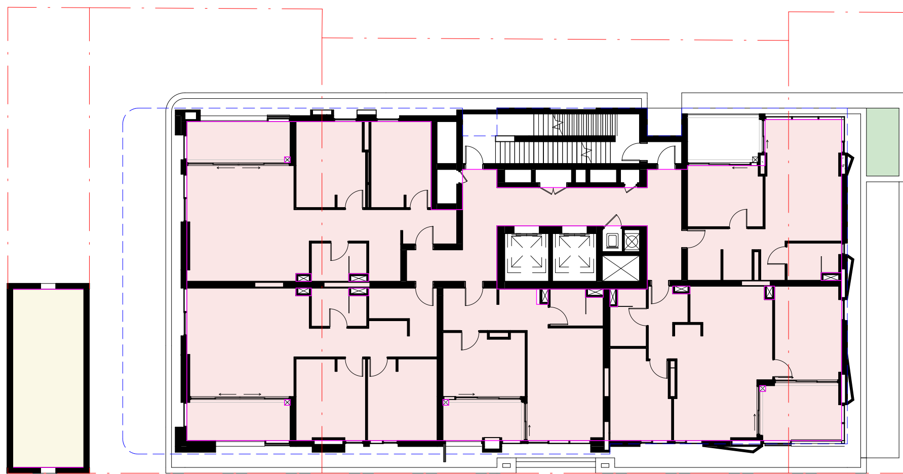
3 LEVEL 02 - LEVEL 03 1:200
