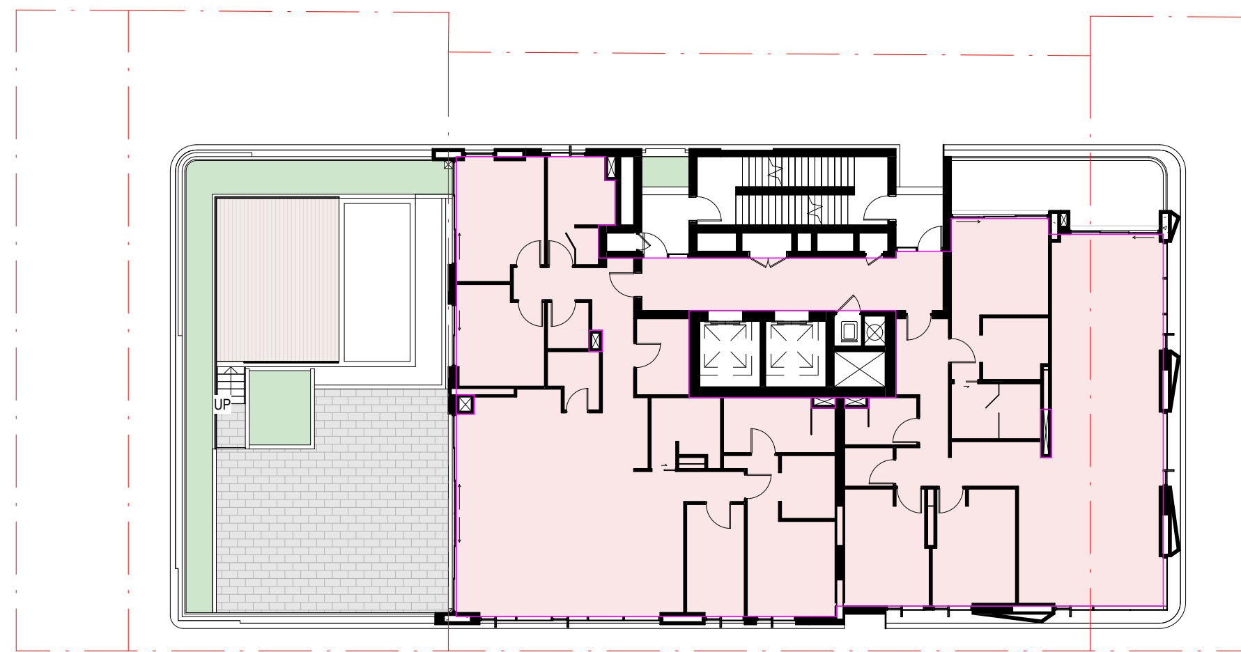
6 LEVEL 11 - LEVEL 12 1:200
