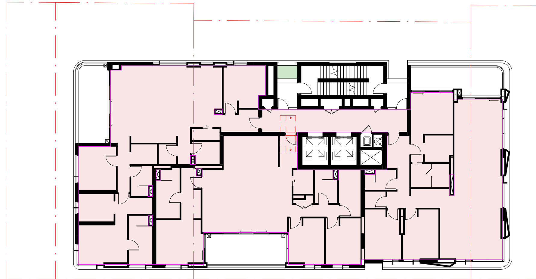
5 LEVEL 06 - LEVEL 10 1:200
