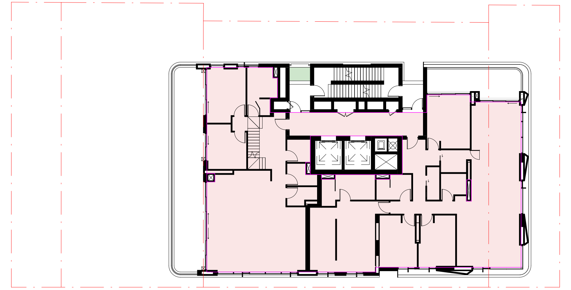
8 LEVEL 12 DA201 1:200
