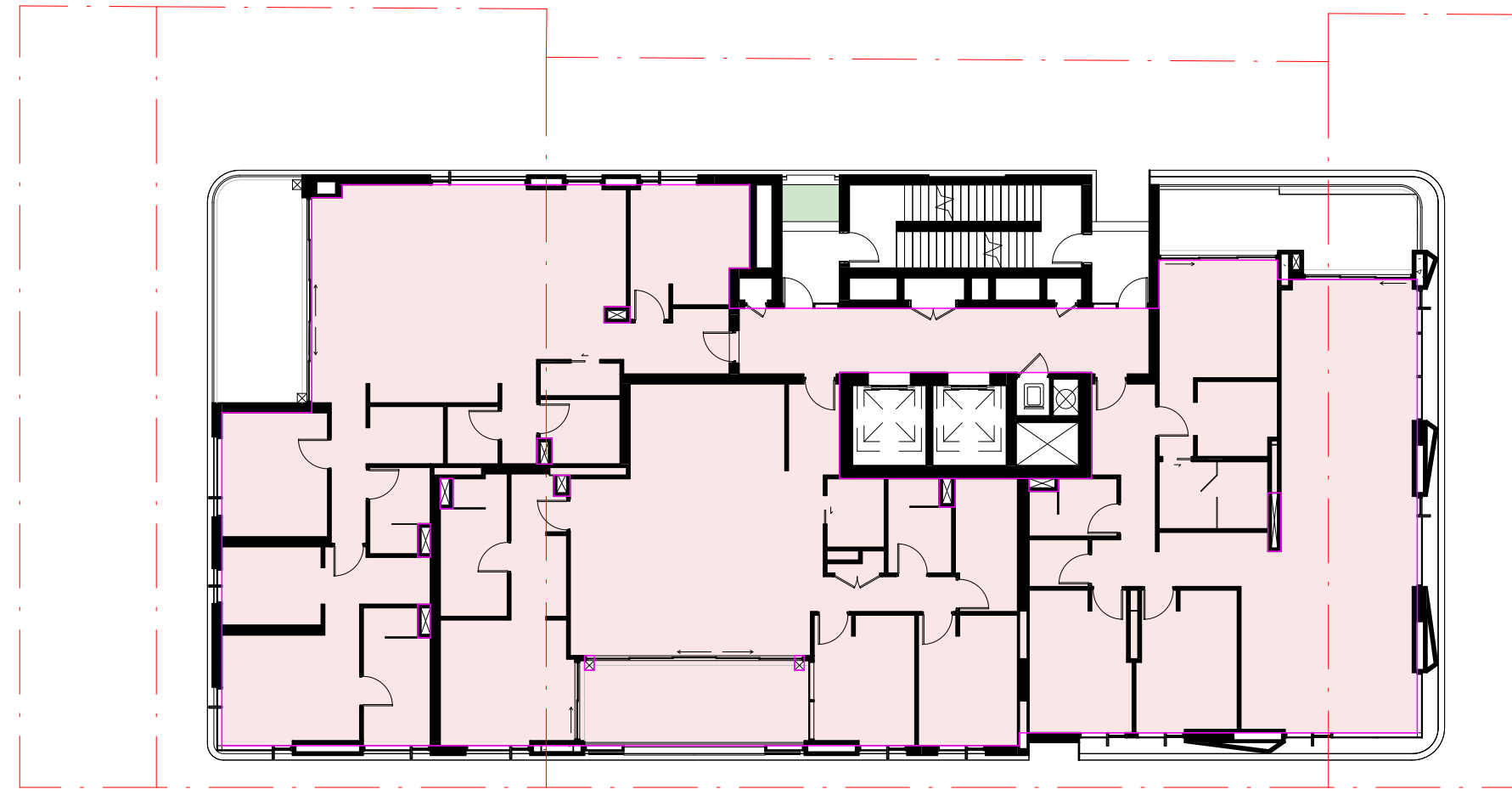
4 LEVEL 04 - LEVEL 05 1:200
