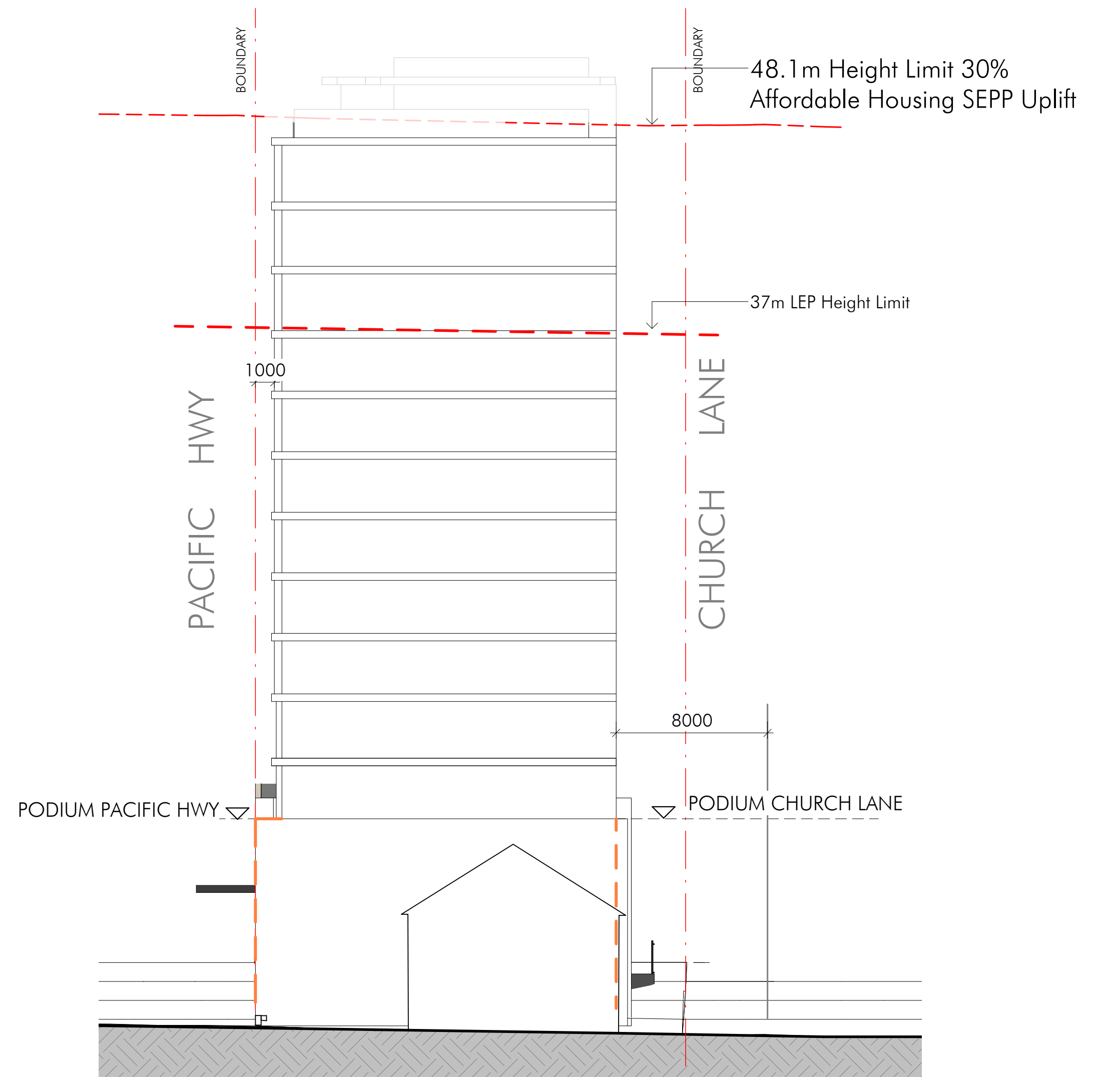
2 101 SSD SOUTH ELEVATION 1: 200
