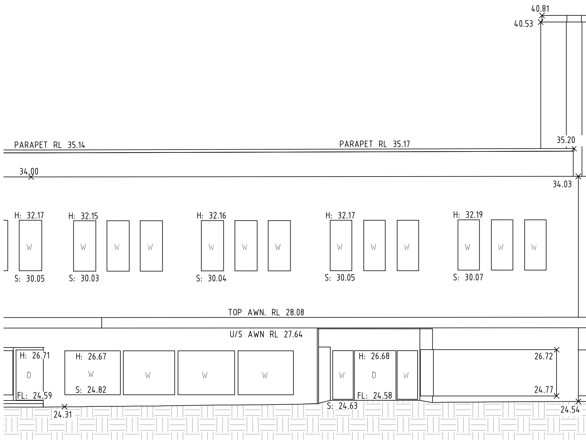
ELEVATION F-F
