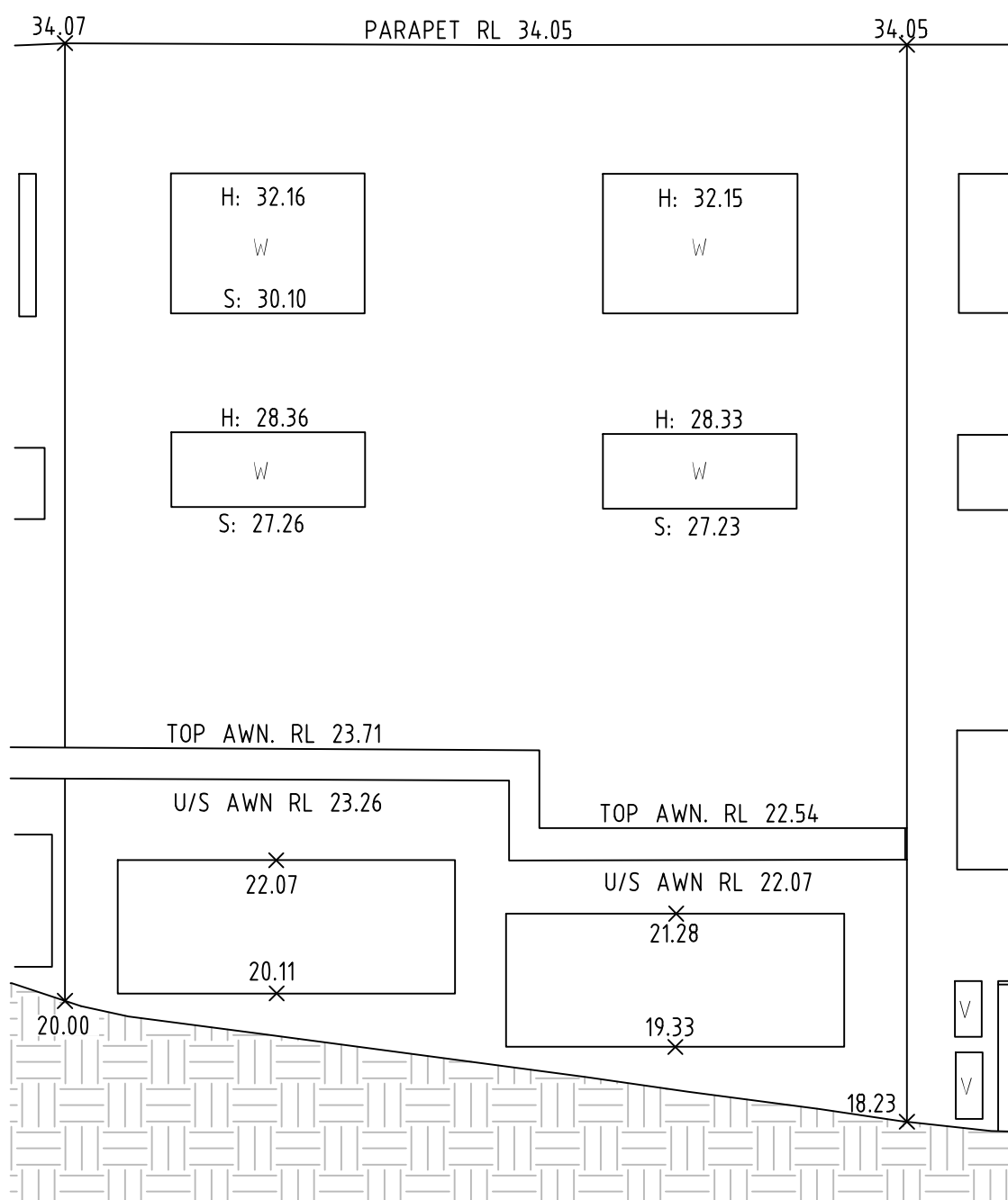
ELEVATION J-J
