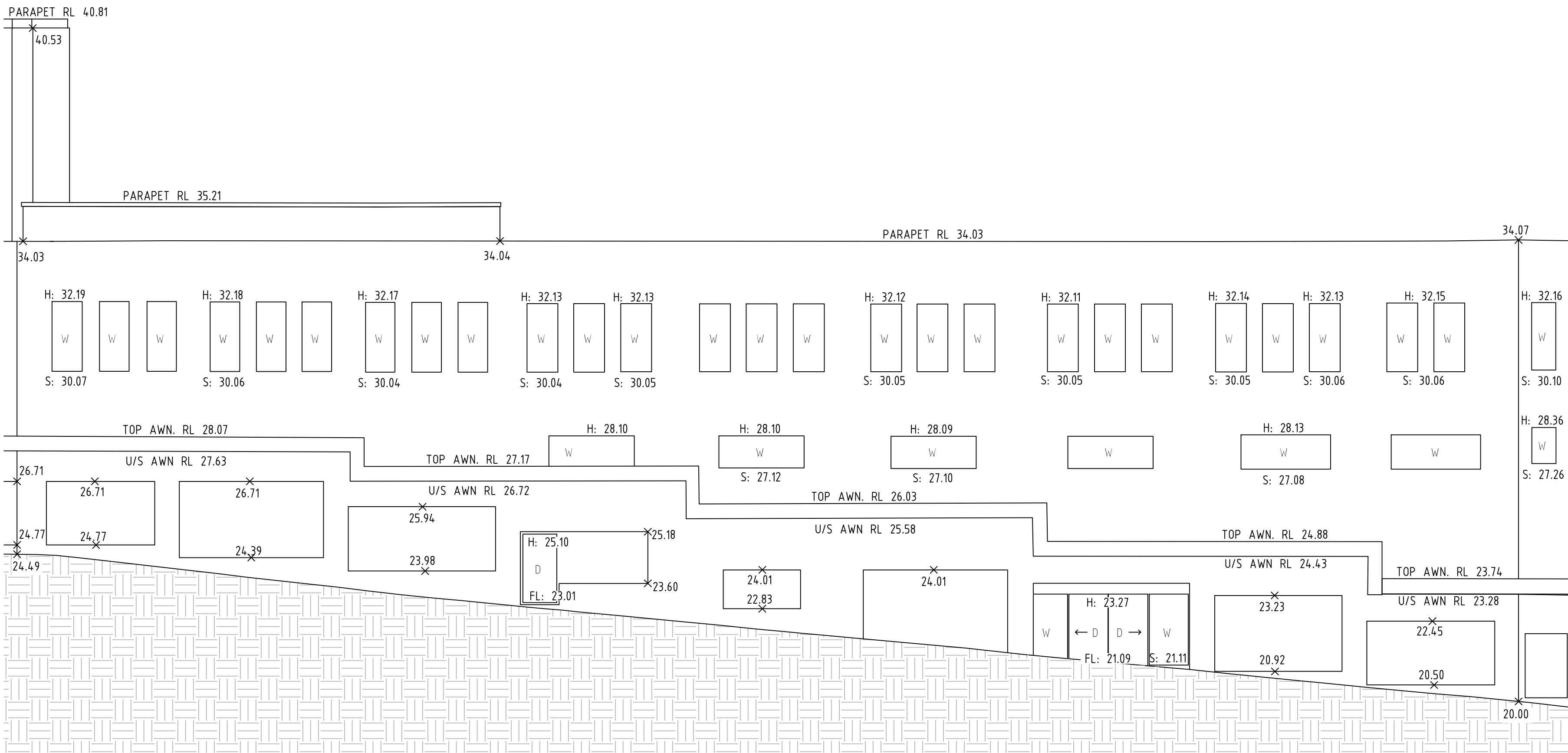
ELEVATION H-H
