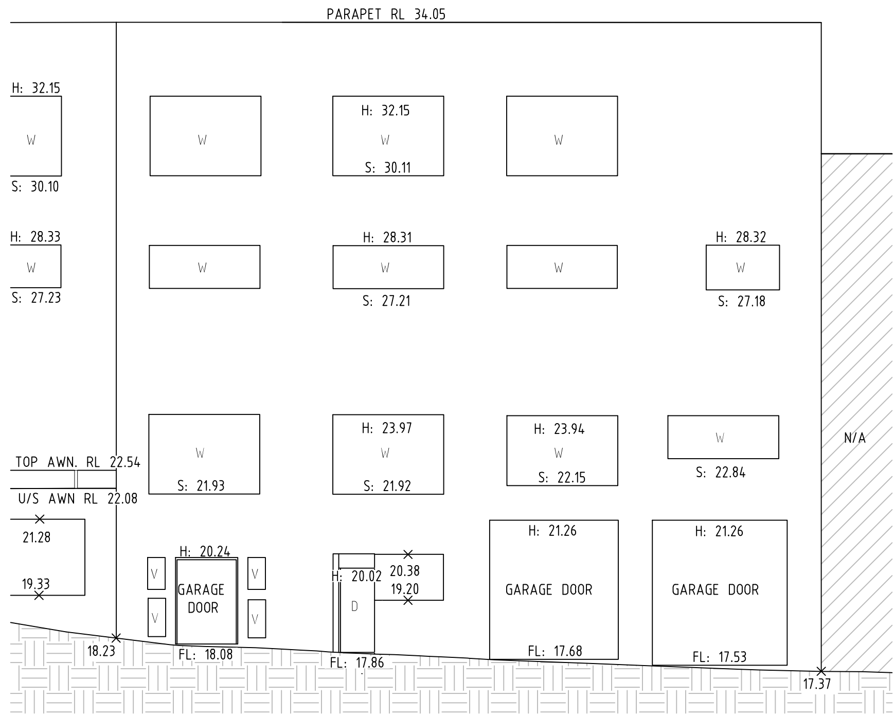
ELEVATION K-K
