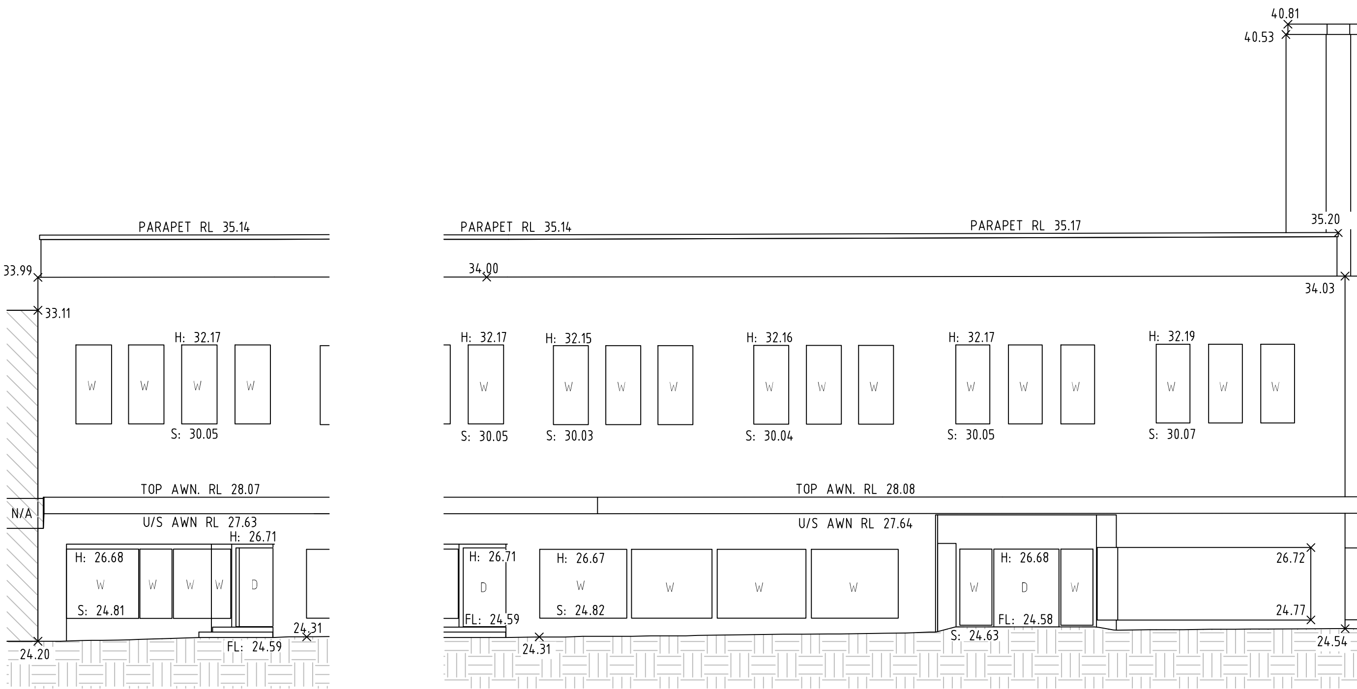
ELEVATION E-E
