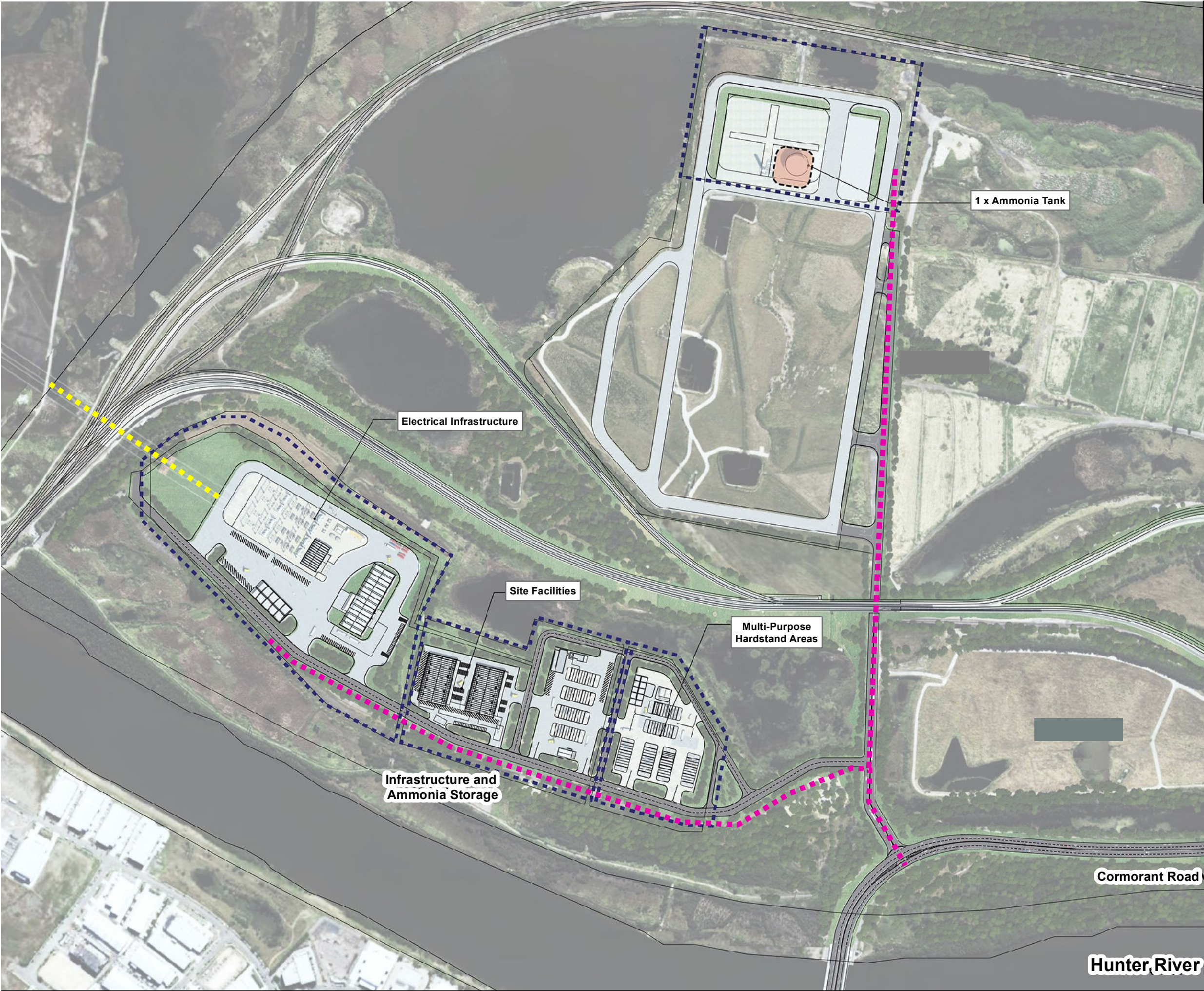
Figure 3-2 Infrastructure and Ammonia Layout
