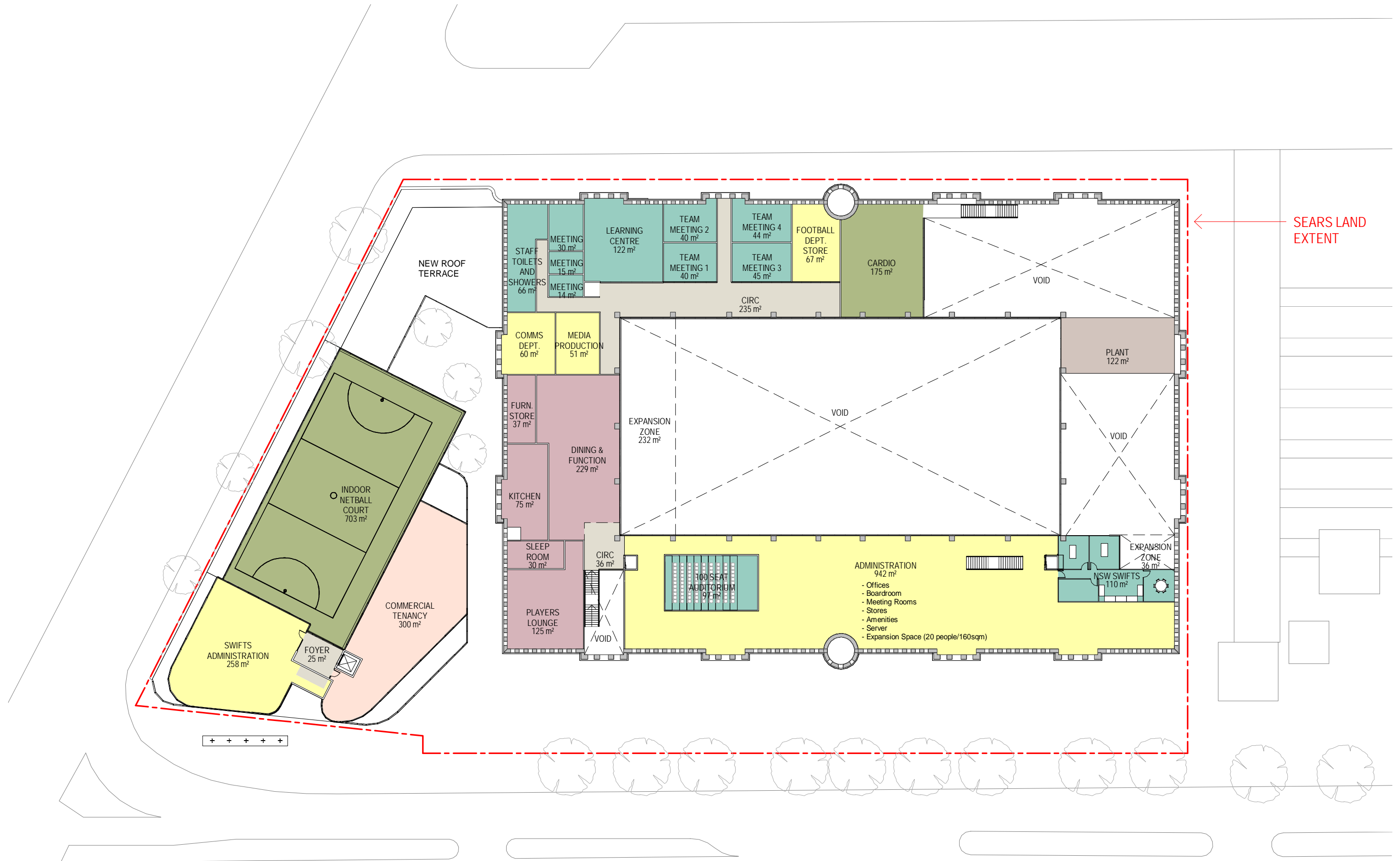
1 PROPOSED FLOOR PLAN - LEVEL 01 1 : 500
