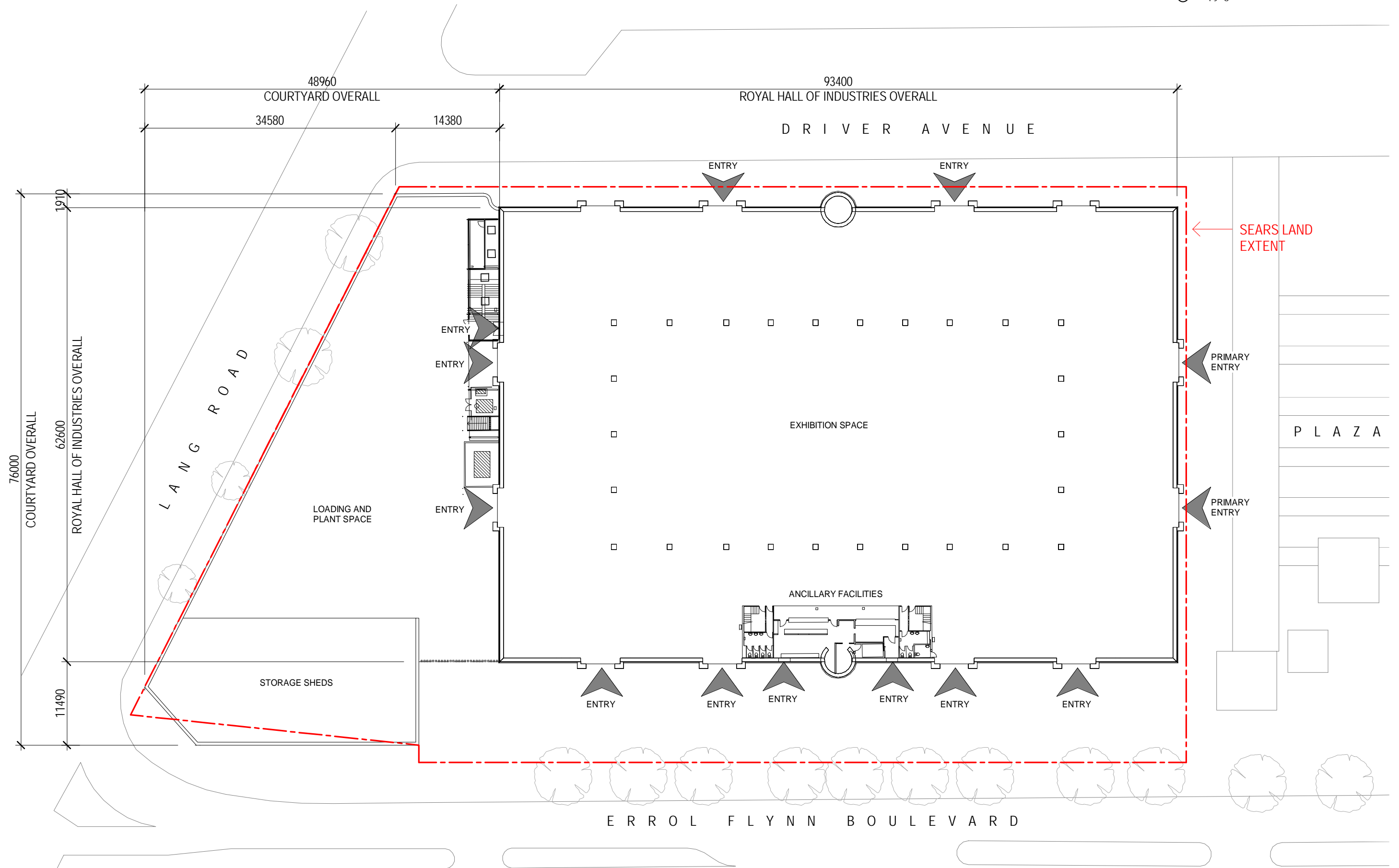
1 EXISTING FLOOR PLAN - GROUND 1 : 500
