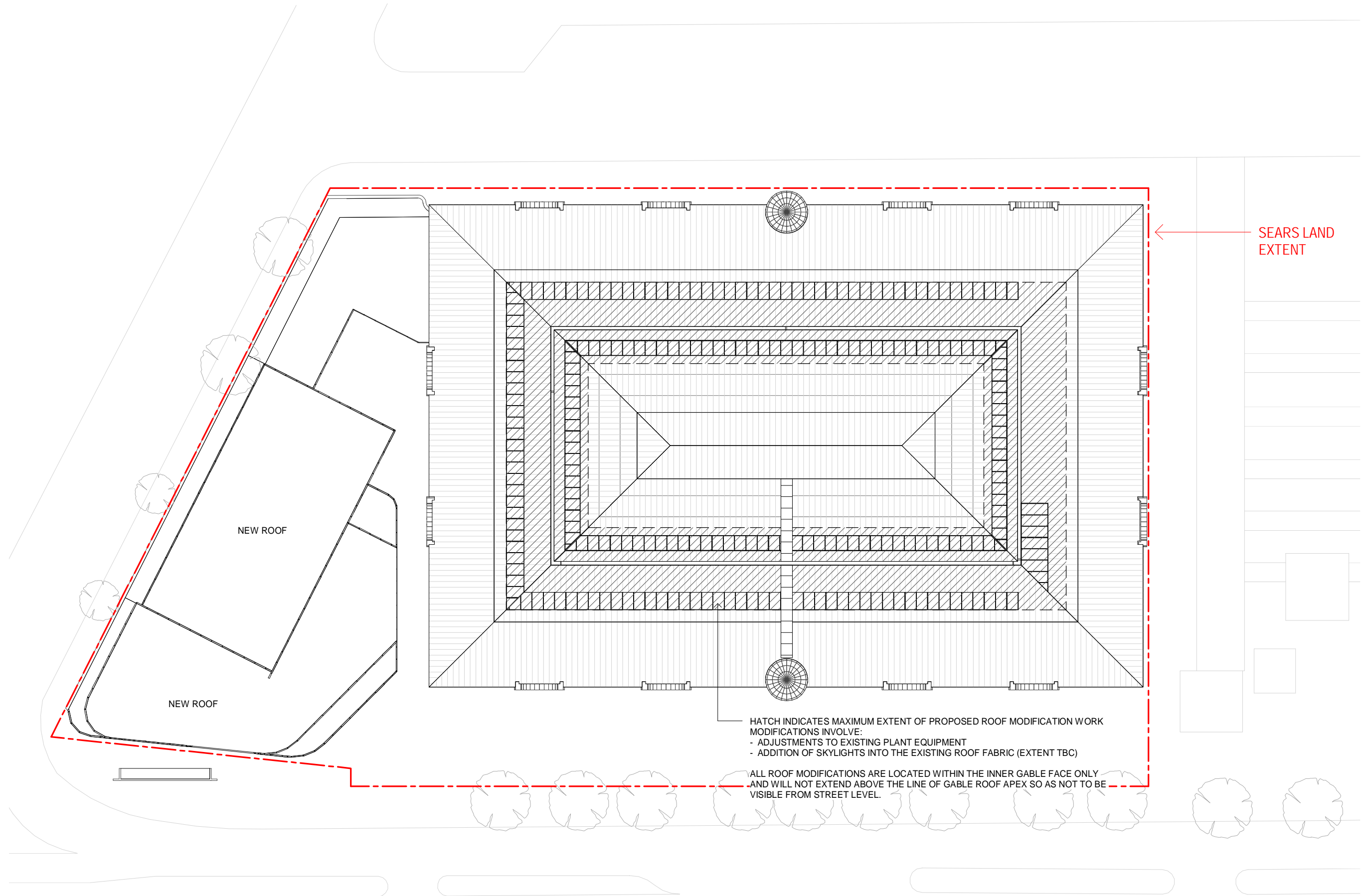
1 PROPOSED FLOOR PLAN - ROOF 1 : 500
