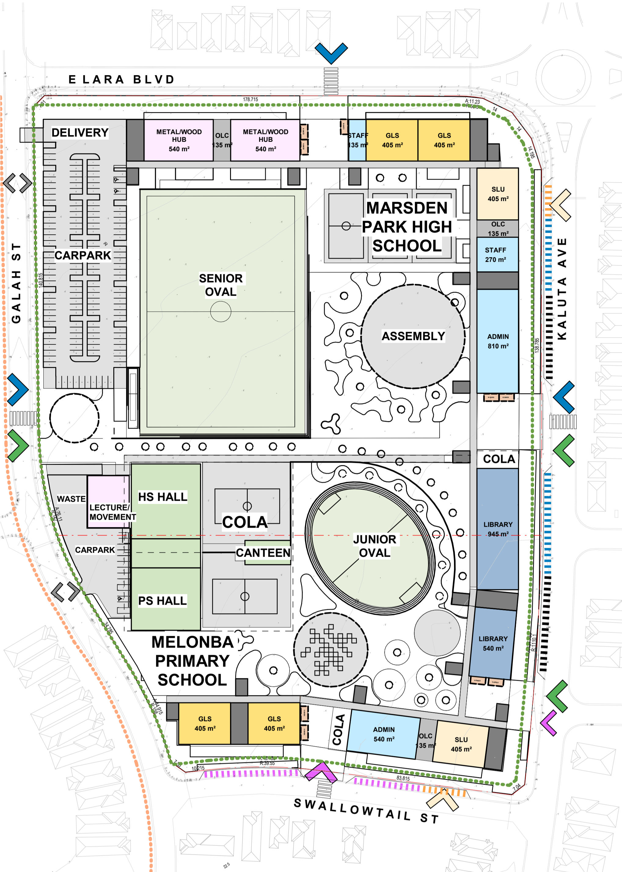
1 GROUND FLOOR - OPTION 5 SDRP 1 : 1000
