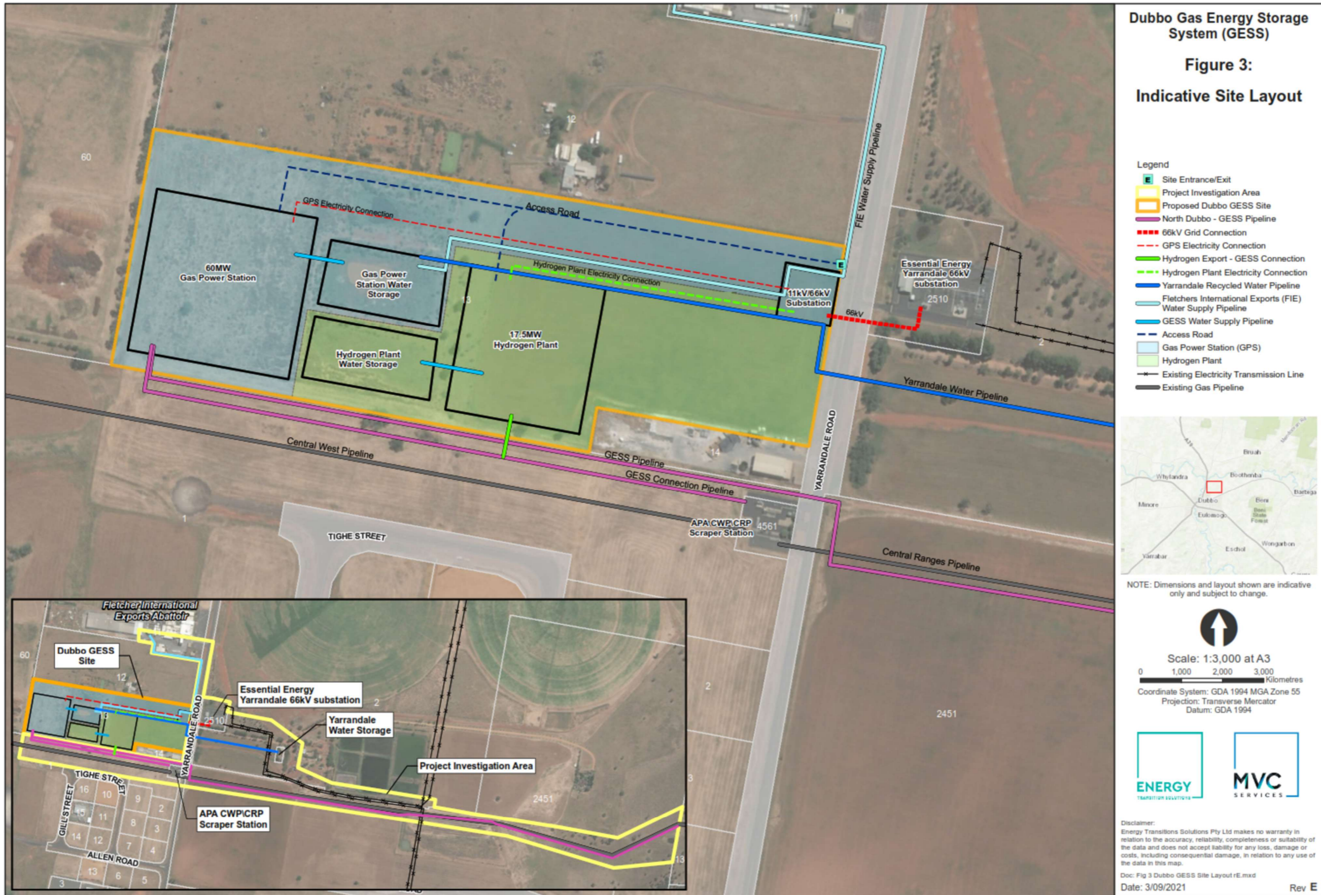
Figure 3. Dubbo GESS indicative site layout
