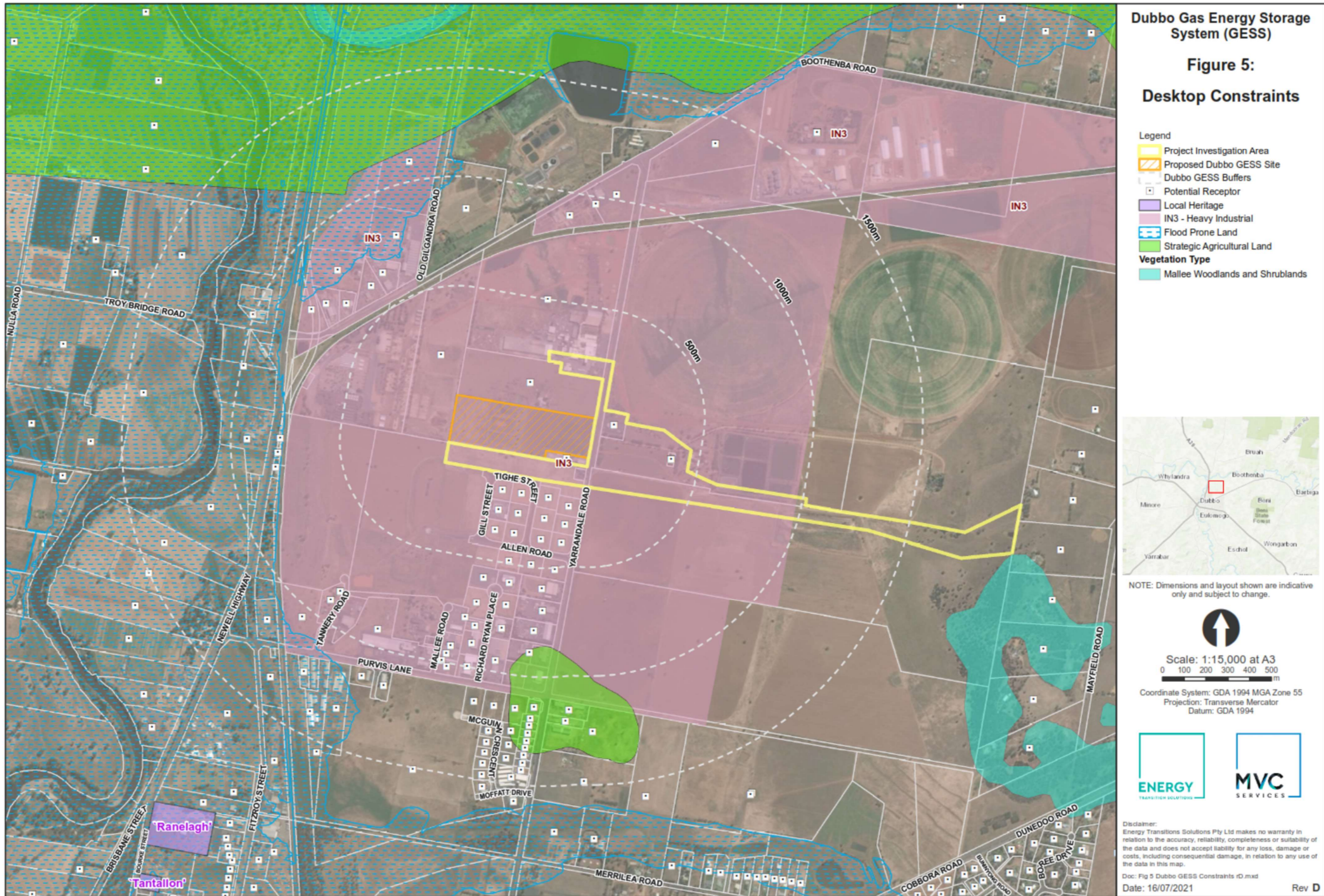
Figure 5. Dubbo GESS site desktop constraints analysis
