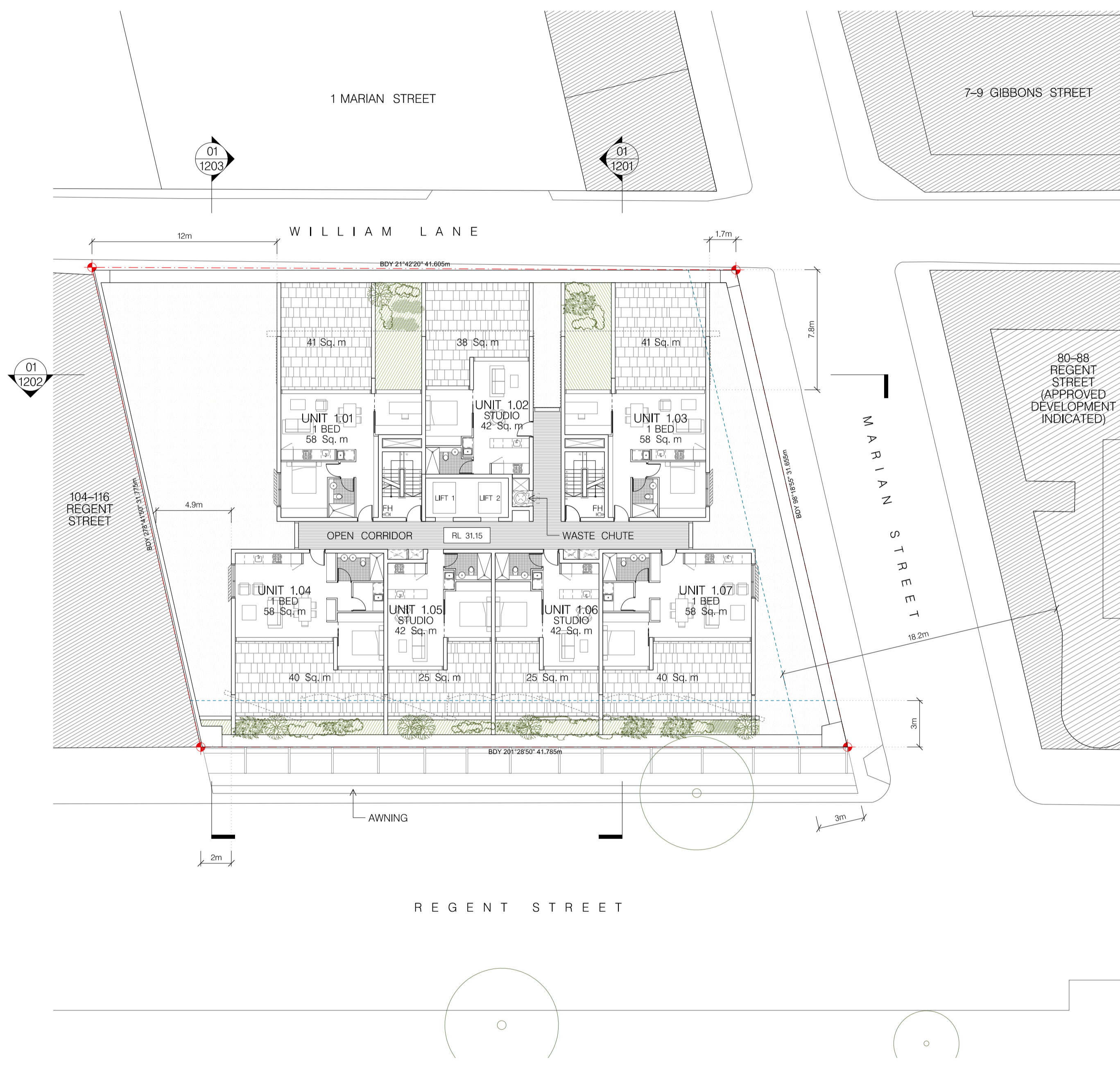
01 LEVEL 1 FLOOR PLAN 1:200
