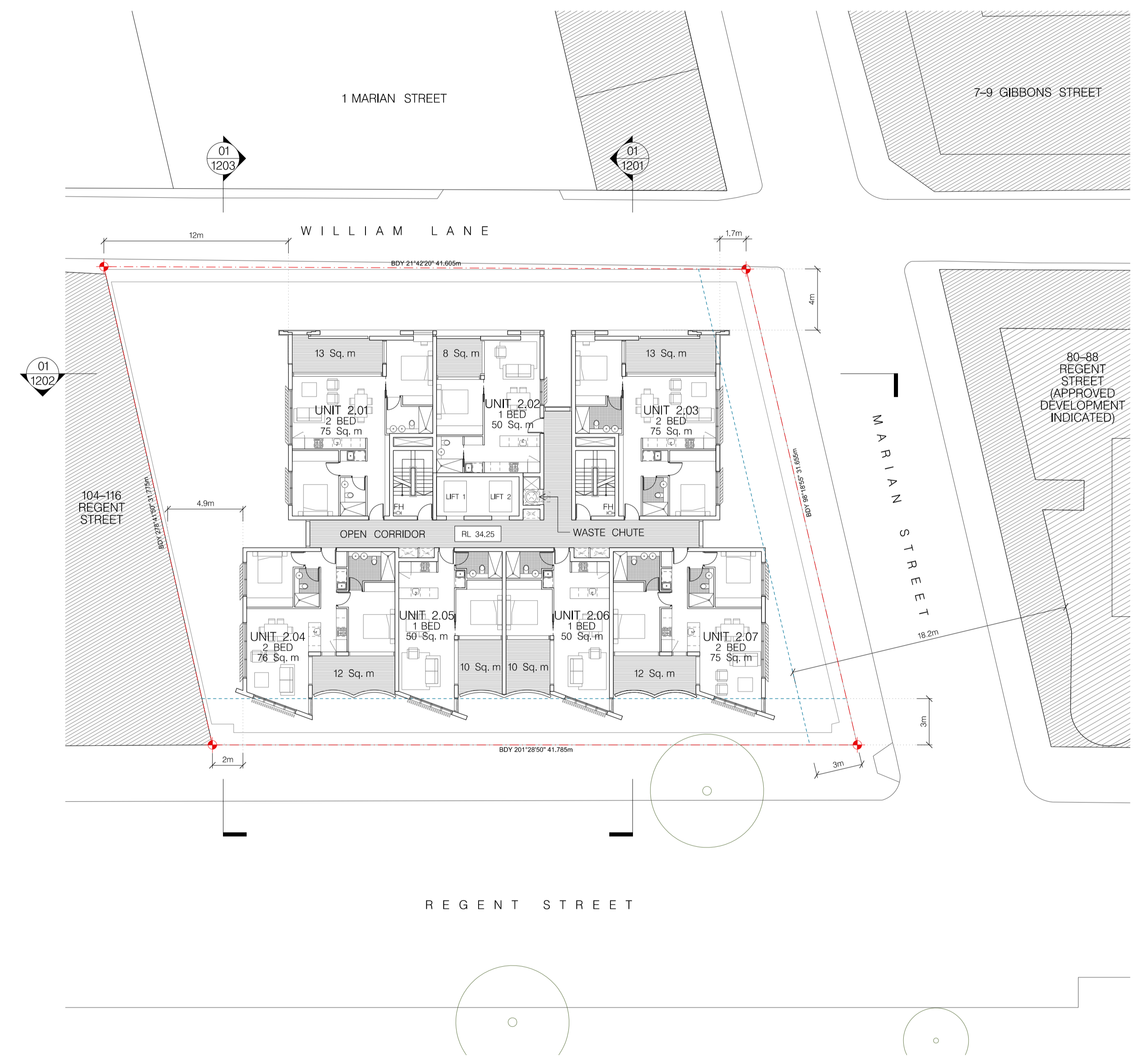
02 TYPICAL LEVEL FLOOR PLAN (LEVEL 2-16) LEVEL 2 SHOWN 1:200
