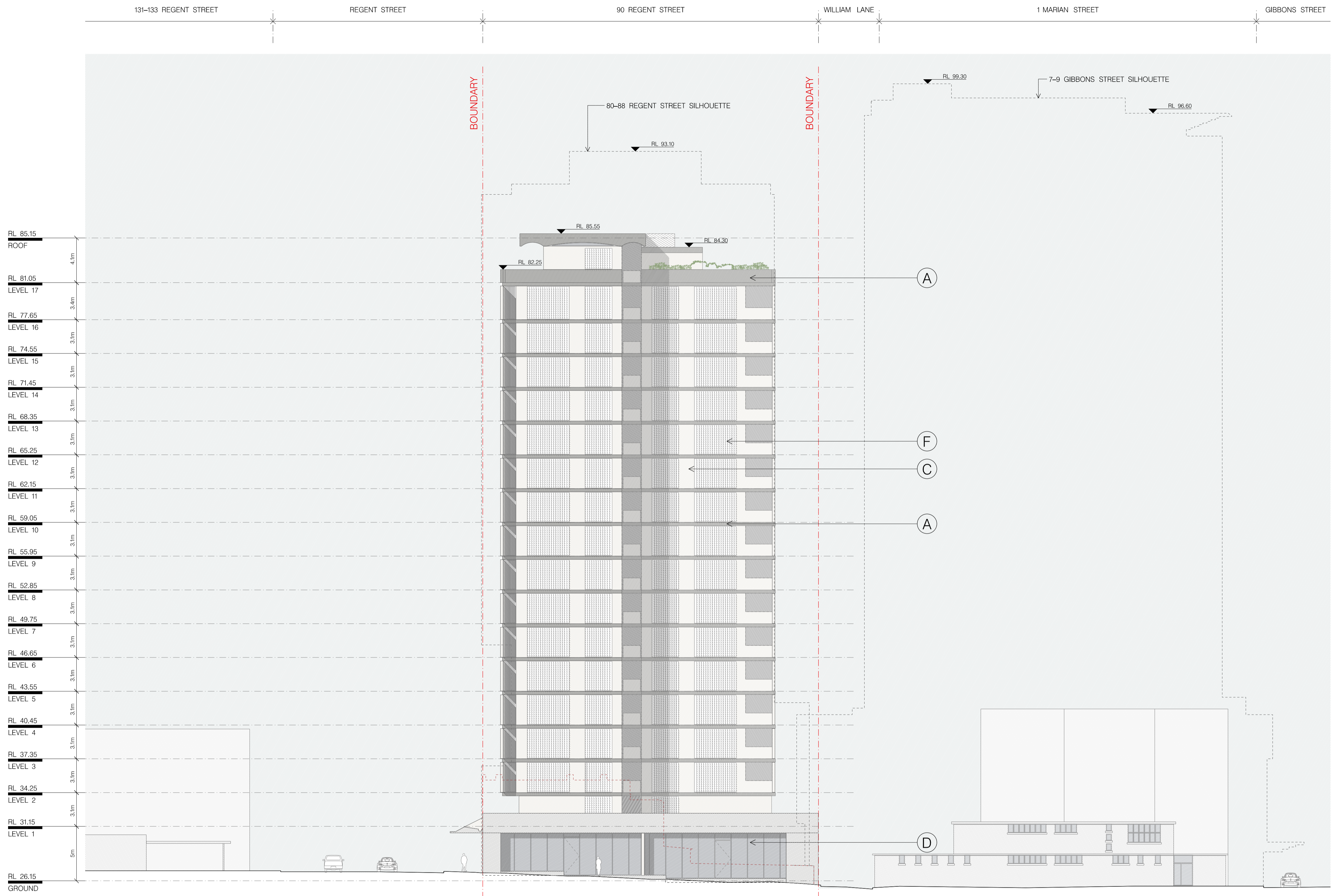
01 NORTH ELEVATION 1:200
