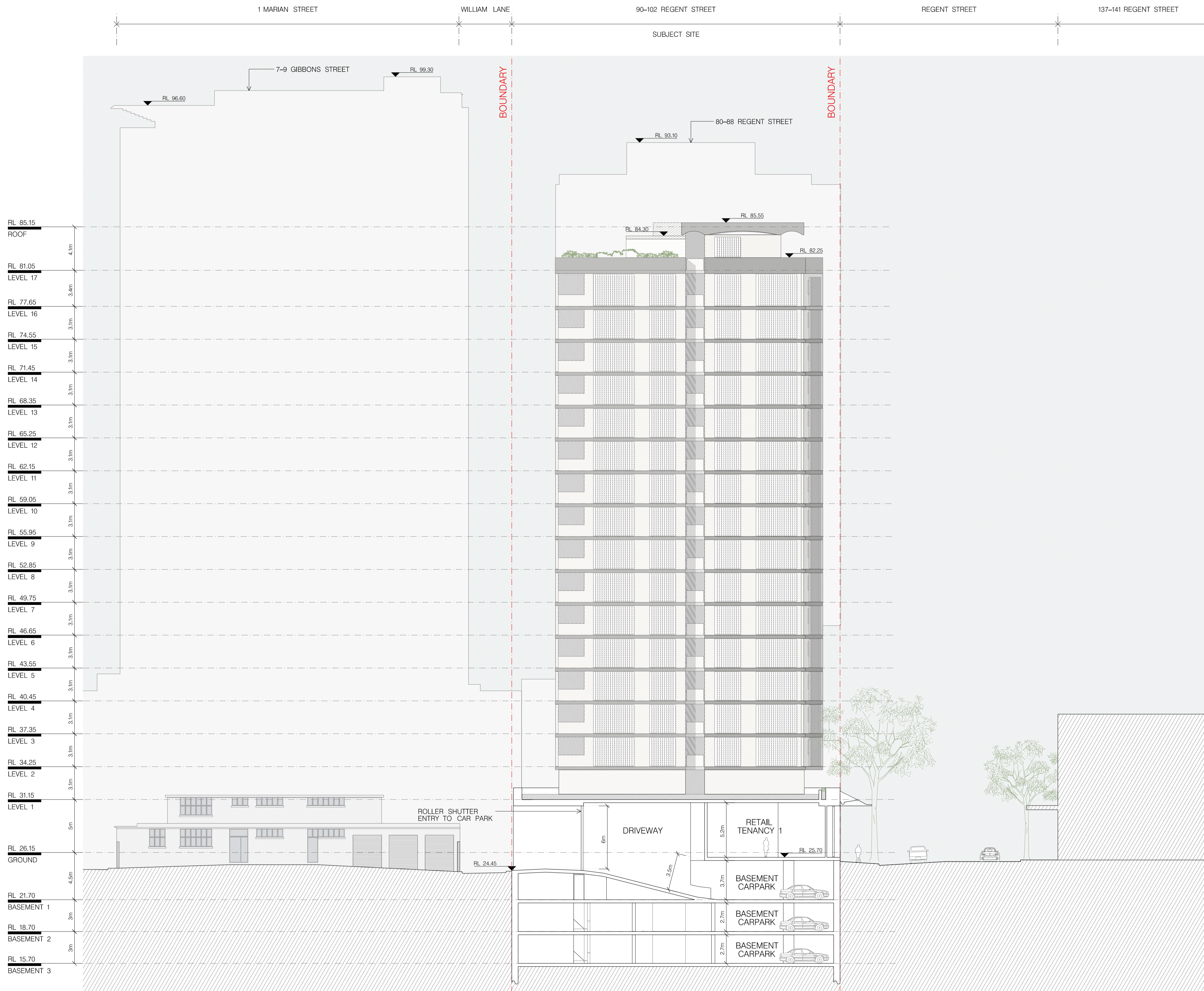
01 SECTION C 1:200
