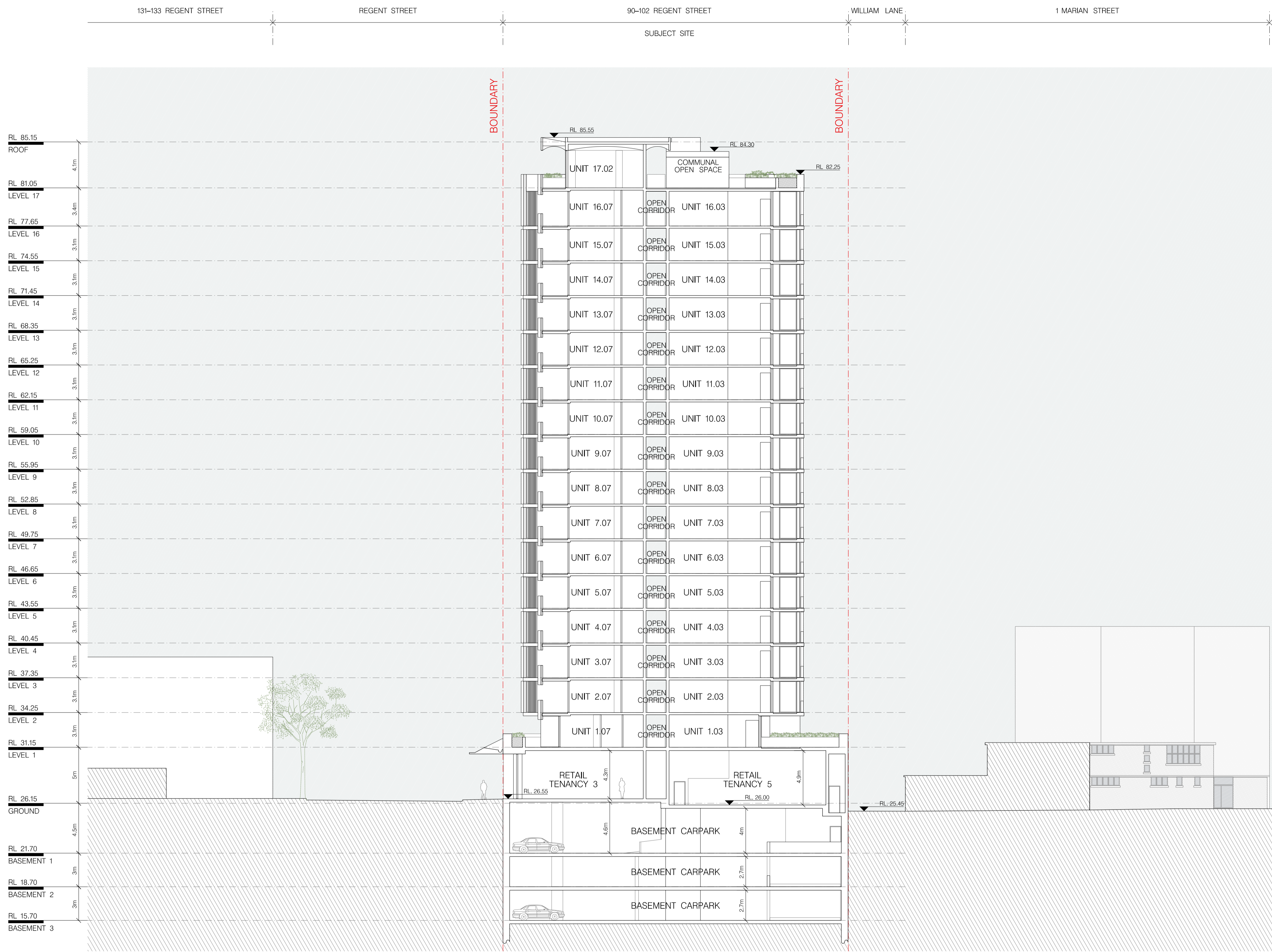
01 SECTION A 1:200
