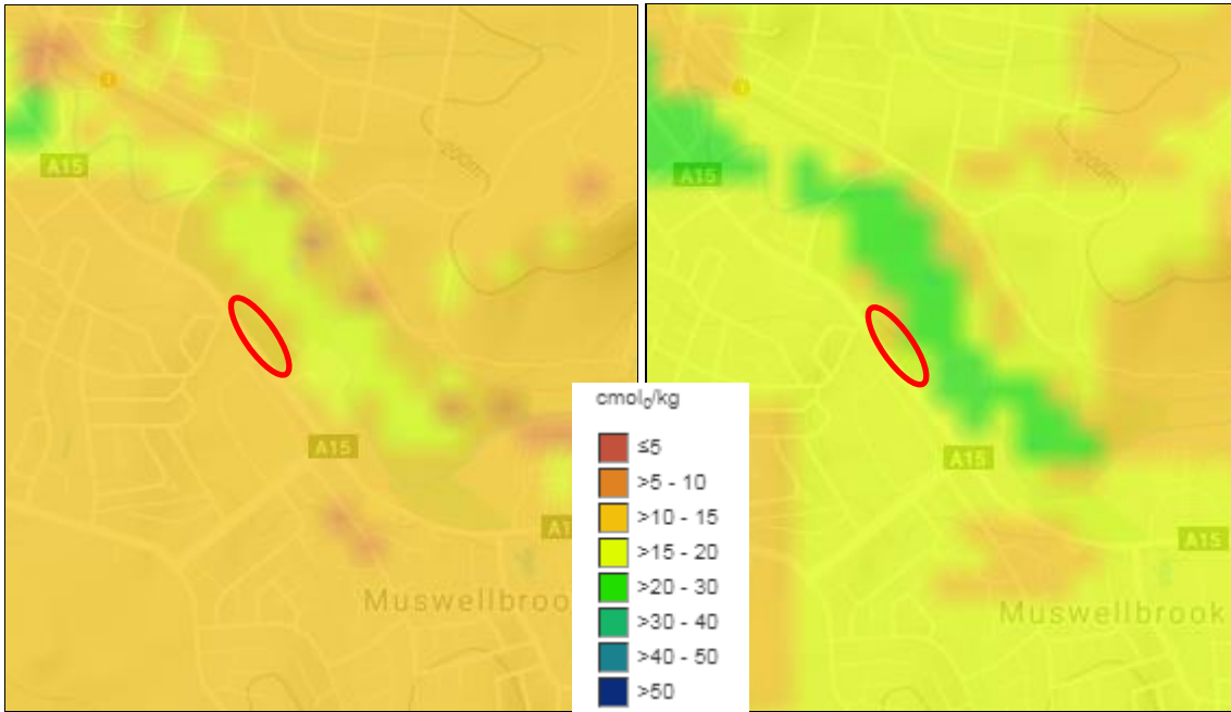
Figure 2: Modelled cation exchange capacity with approximate site location (red outline)
