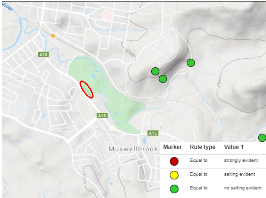
Figure 1: Soil profiles with salinity potential with approximate site location (red outline)
