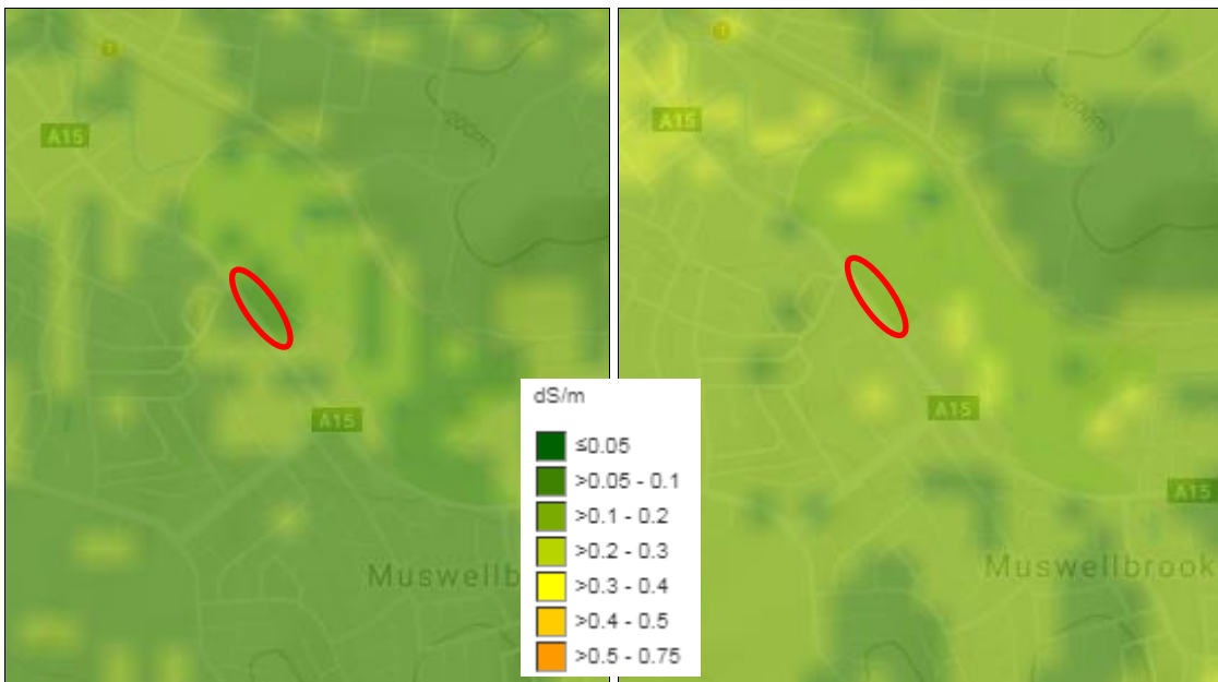
Figure 3: Modelled electrical conductivity with approximate site location (red outline)
