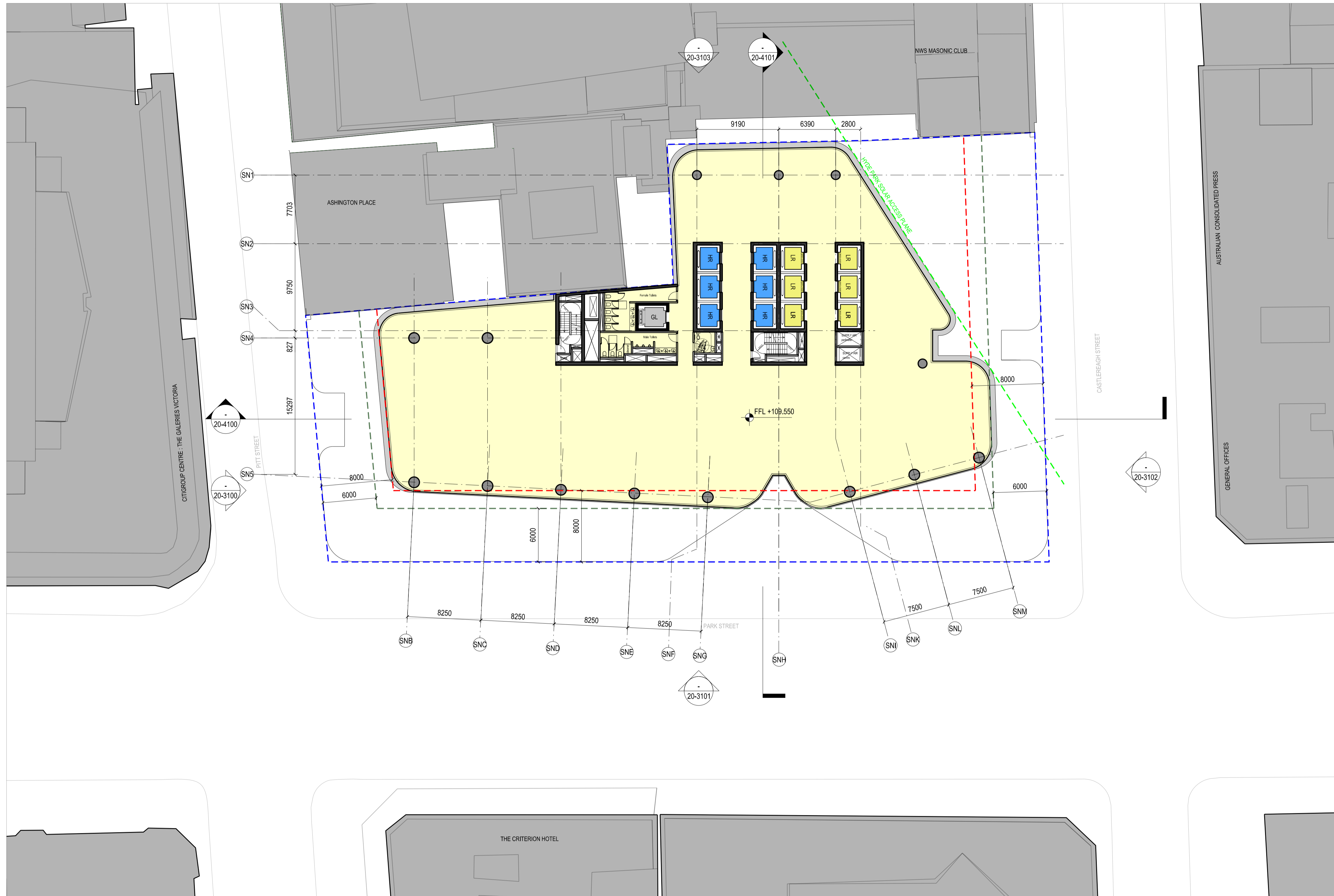
01 TOWER LEVEL 13 PLAN 1:250
