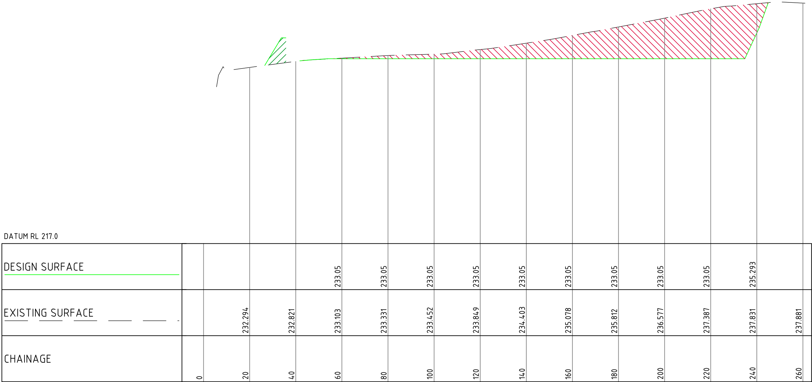
LONGITUDINAL SECTION ALONG 04 HORIZONTAL SCALE 1:1000@A1 VERTICAL SCALE 1:200@A1
