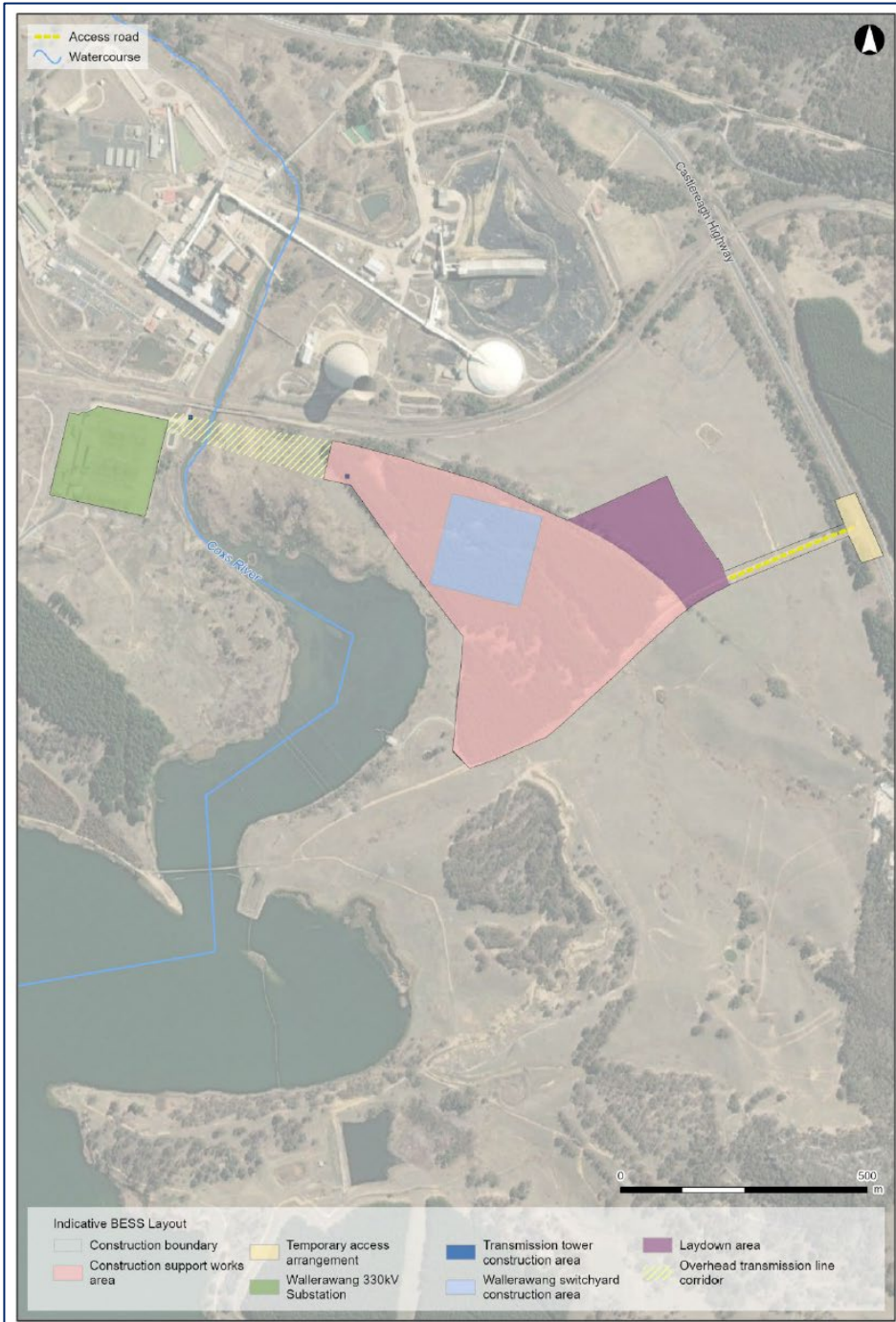
Figure 2: Project Construction Footprint – Battery Energy Storage System BESS
