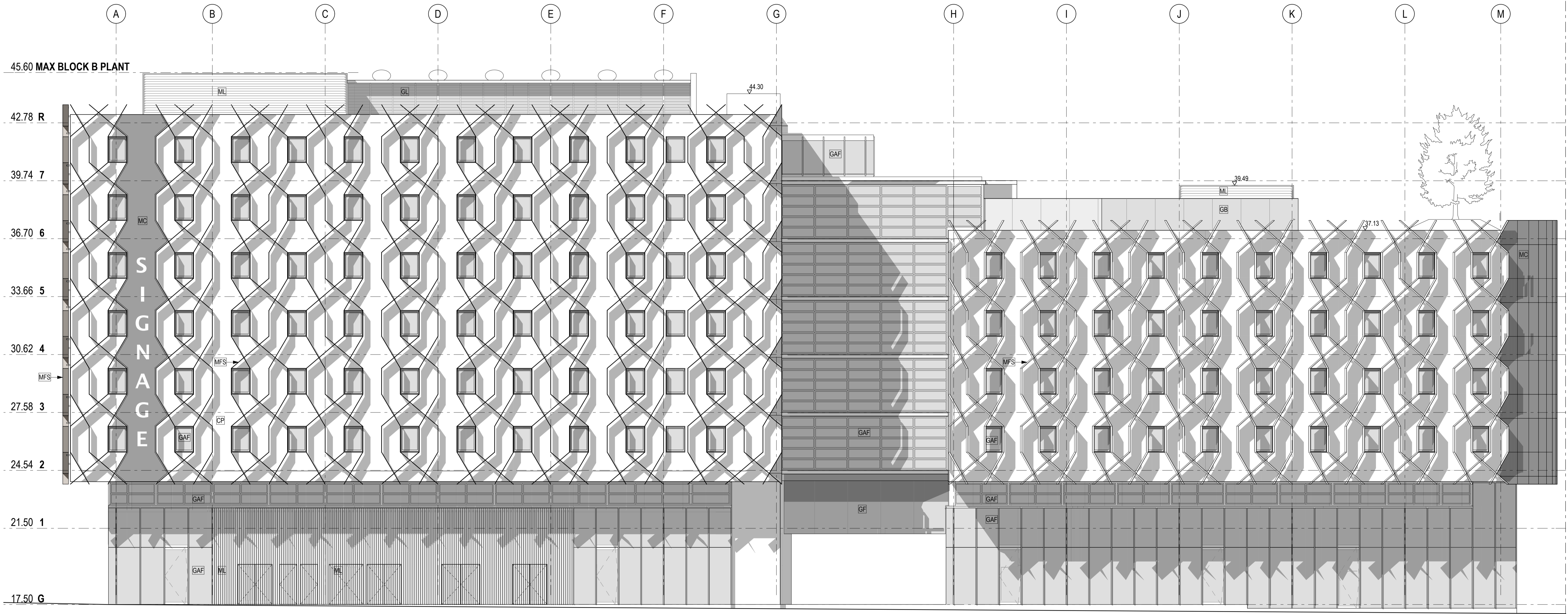
1 WEST ELEVATION
