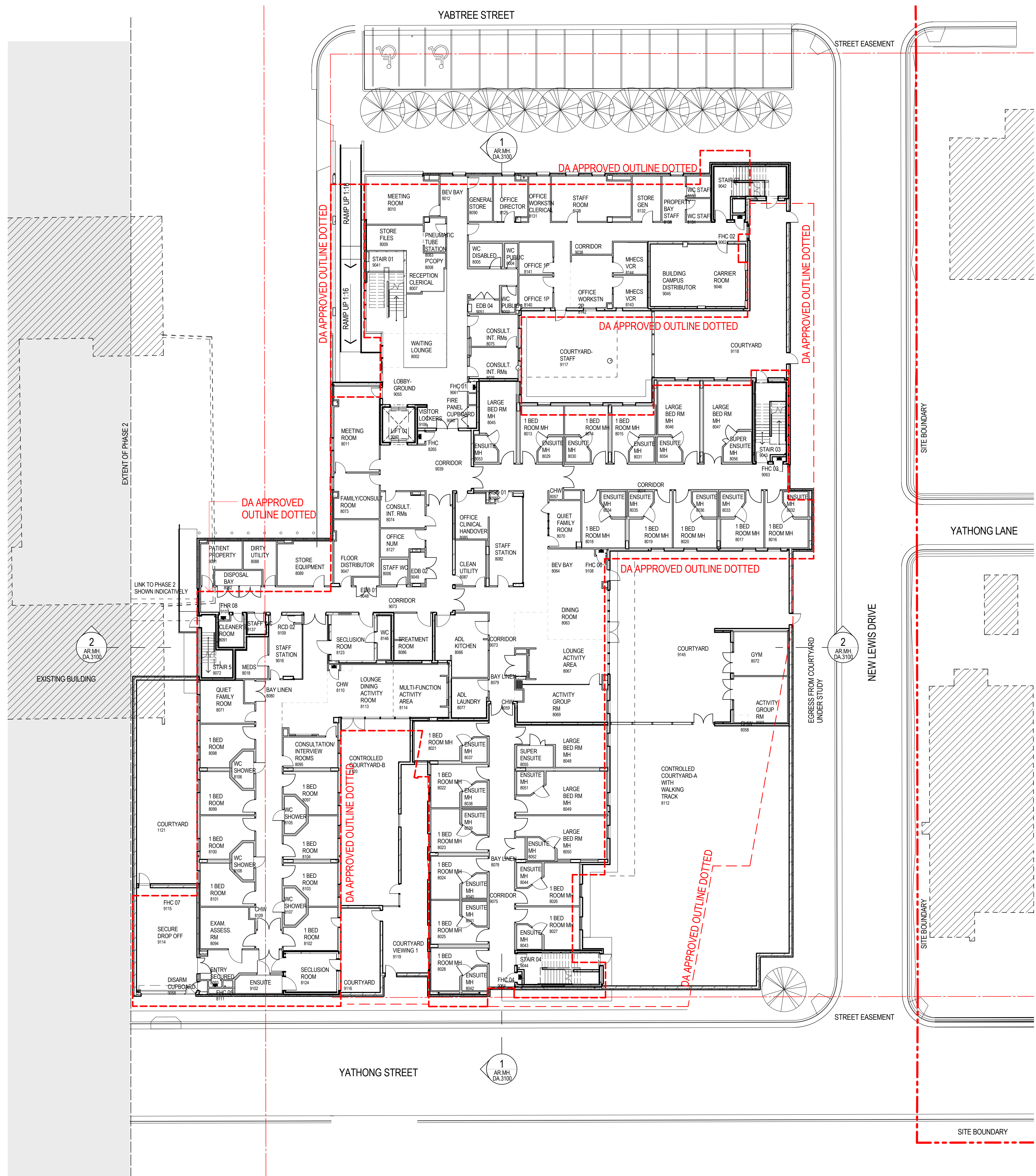
1 GROUND FLOOR GENERAL ARRANGEMENT PLAN SCALE 1:200
