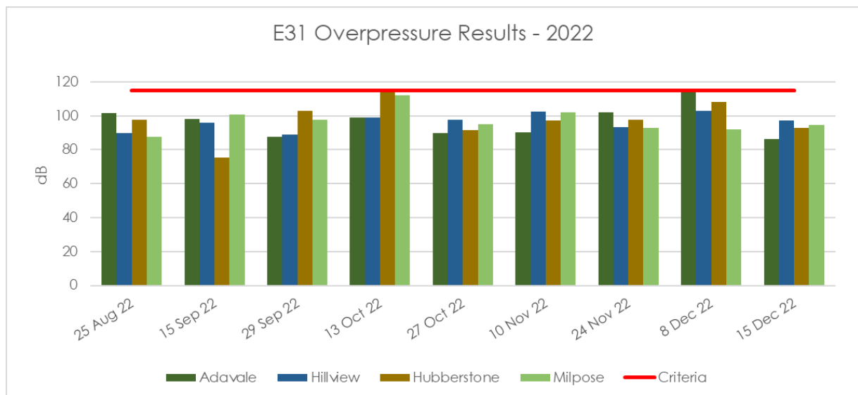
Figure 20 Overpressure results for surface blasting of E31 pit
