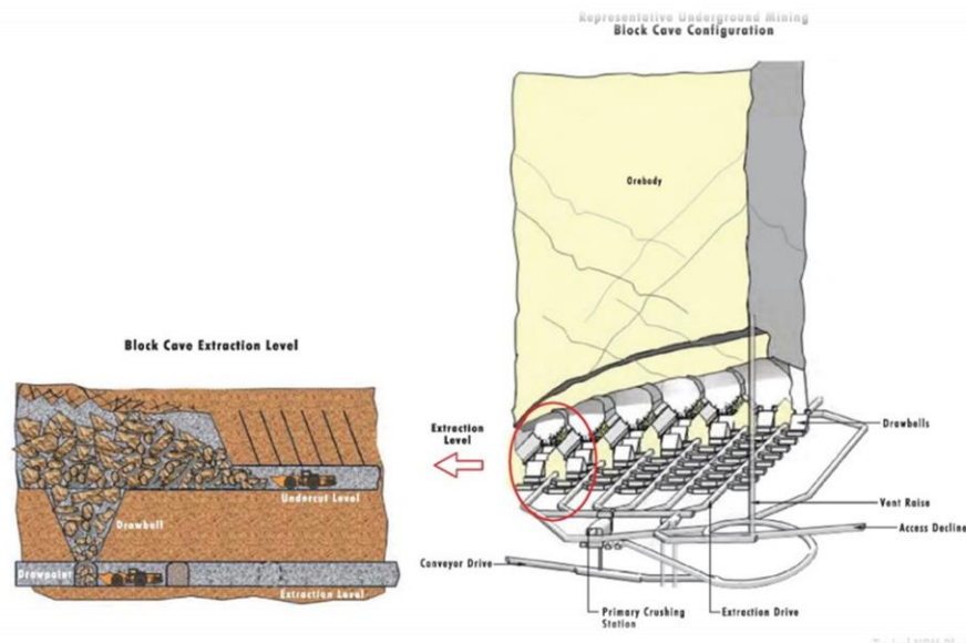
Figure 4 Block Cave Mining Method
