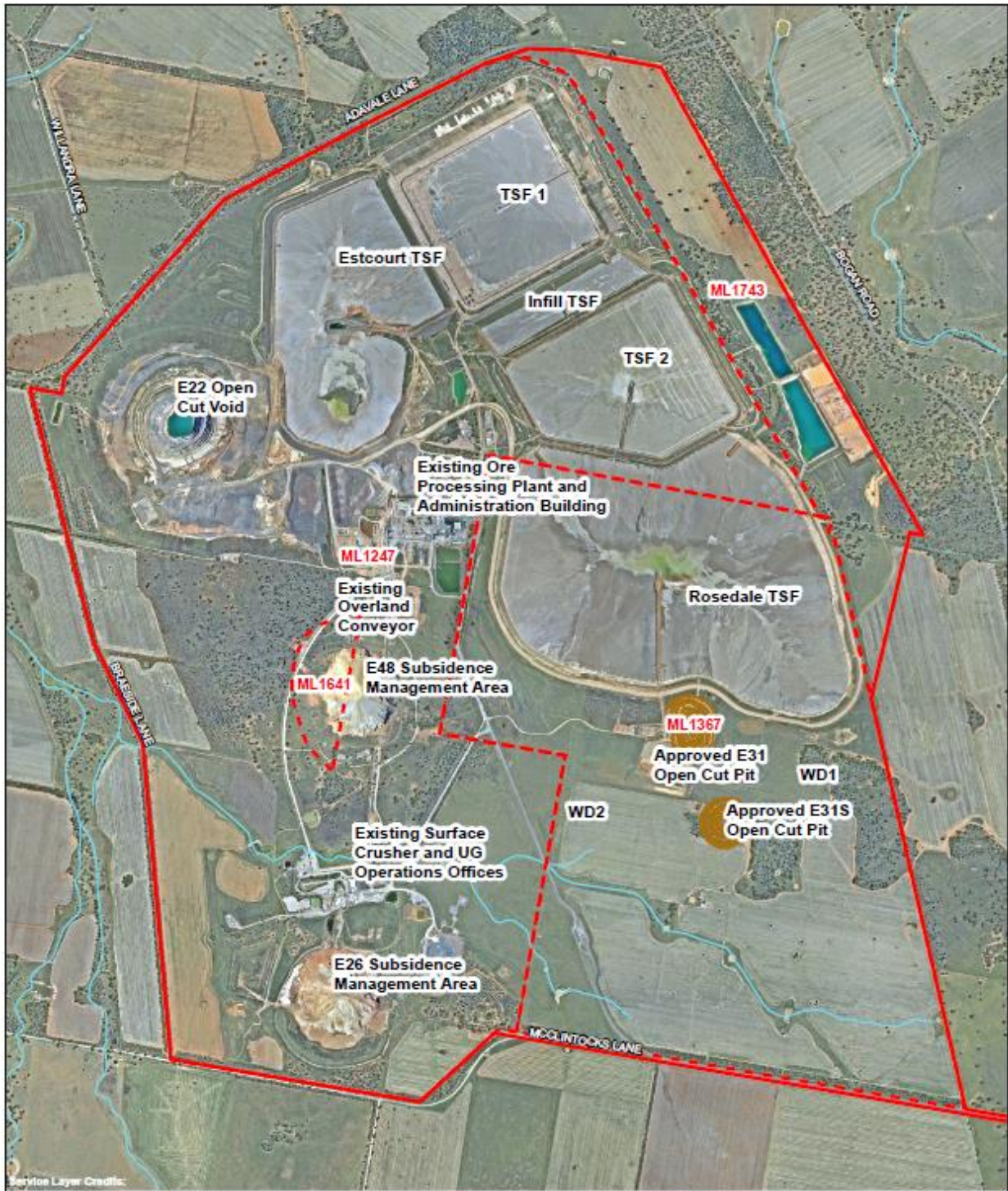
Figure 3 Site features
