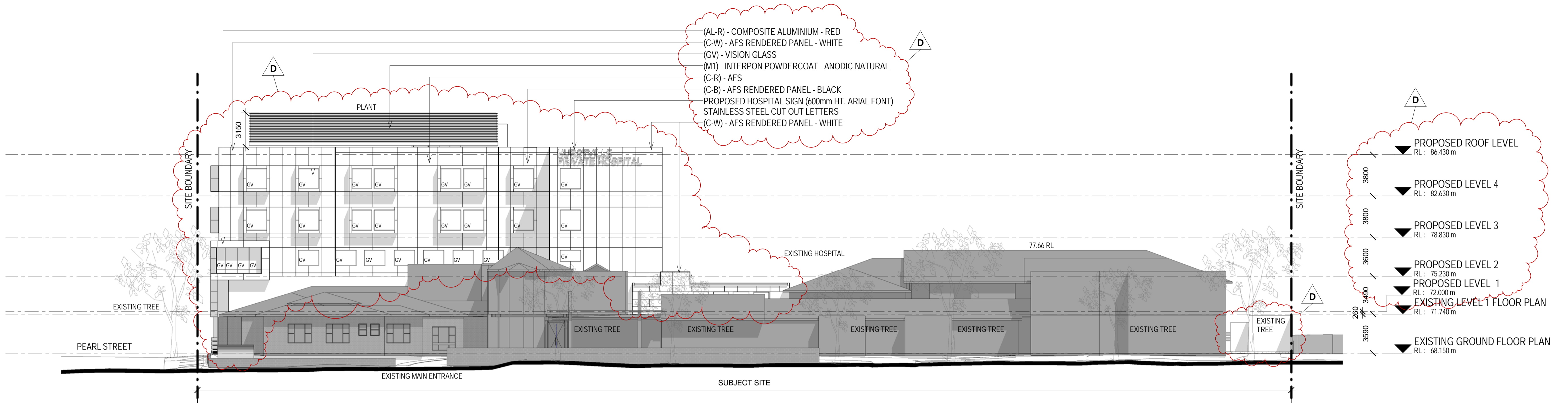
1 GLOUCESTER ROAD - ELEVATION DA-32 Scale 1:200
