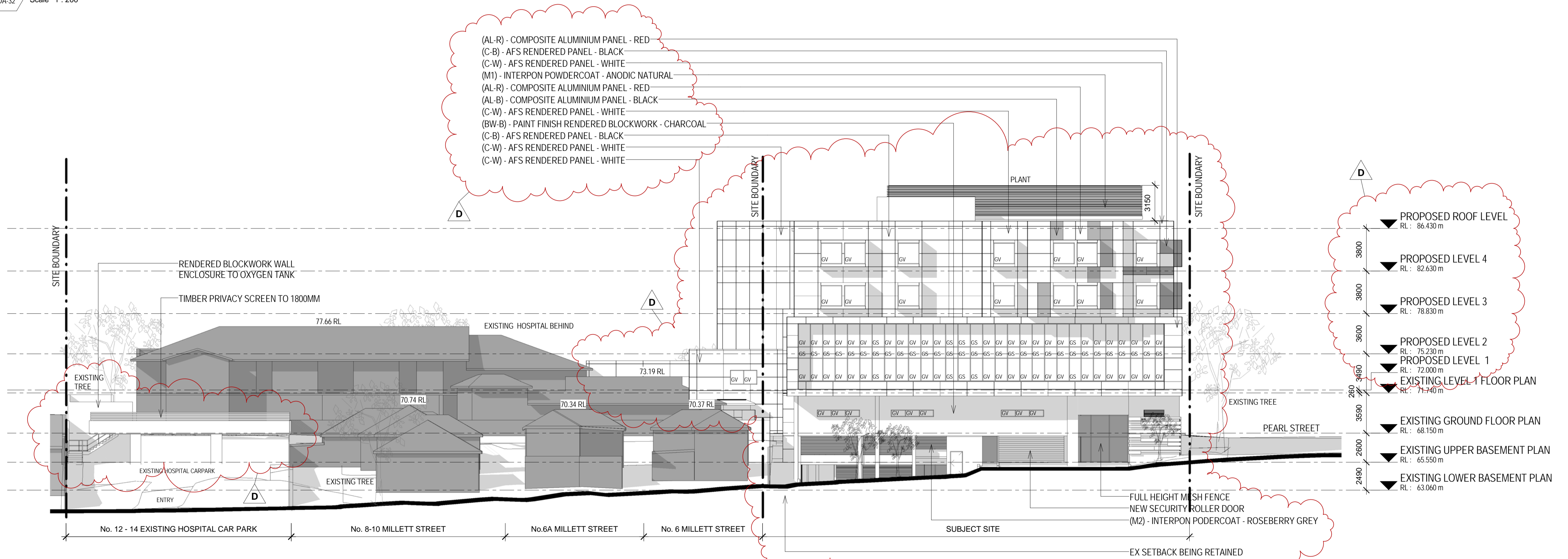
1 GLOUCESTER ROAD - ELEVATION DA-32 Scale 1:200
