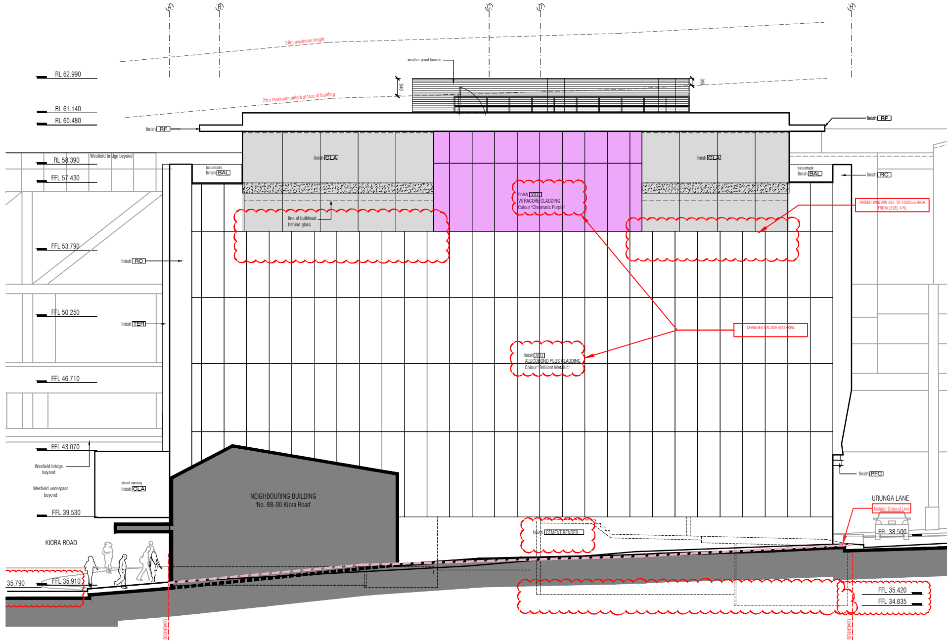
south elevation kiora road scale: 1:100
