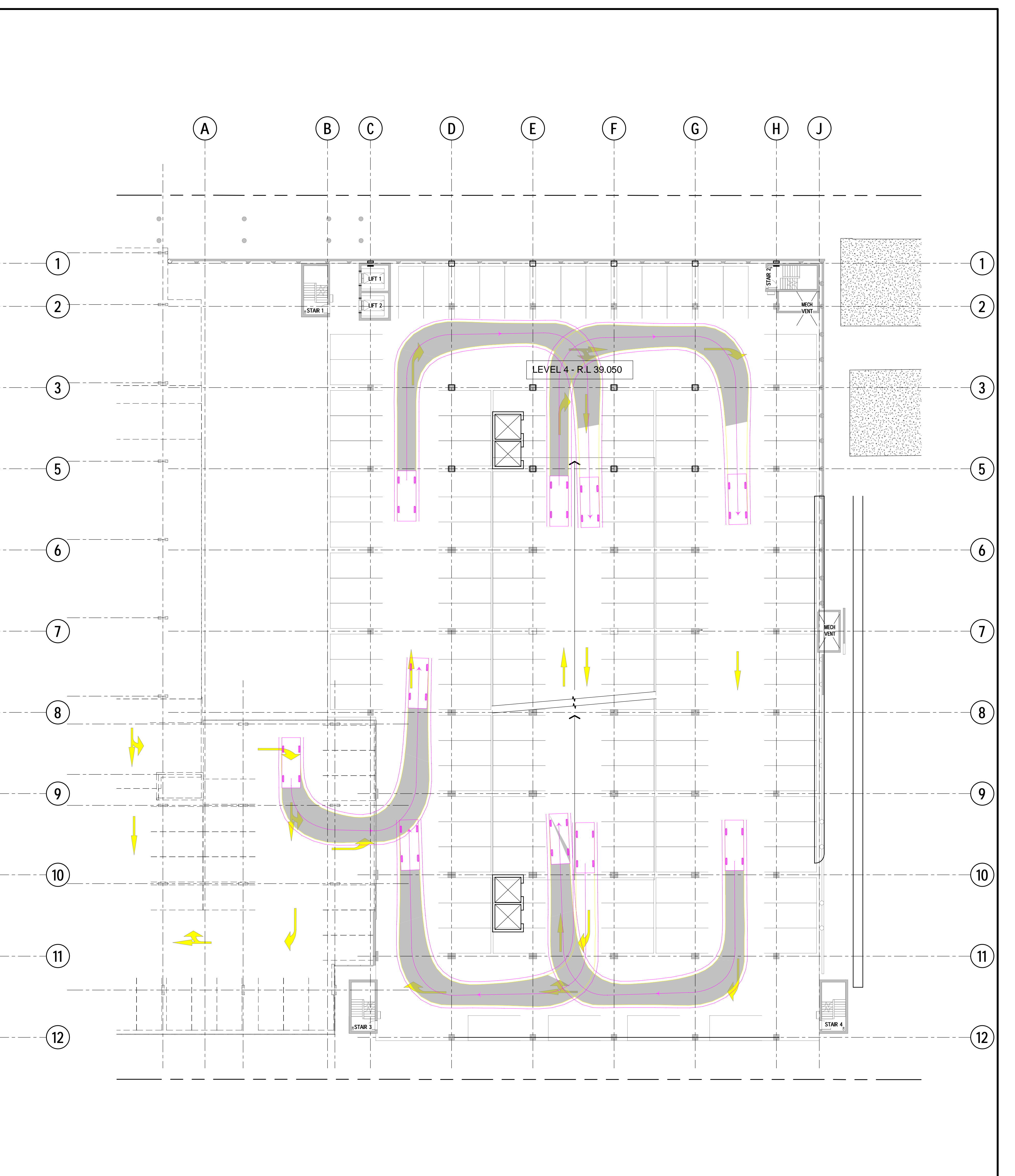
LEVEL 4 - CIRCULATION PLAN - FUTURE EXPANSION SCALE: 1 : 200
