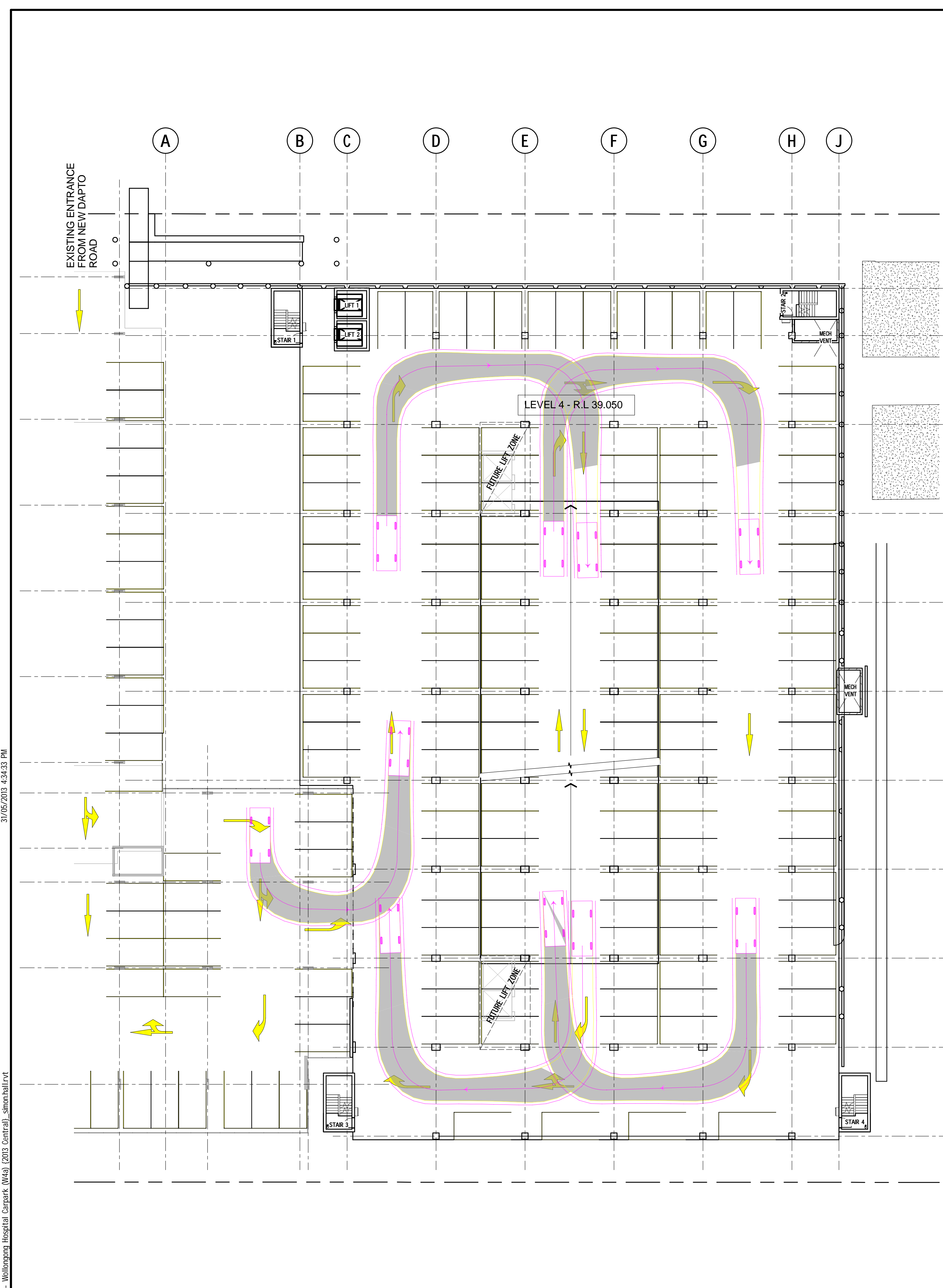
LEVEL 4 - CIRCULATION PLAN SCALE: 1 : 200
