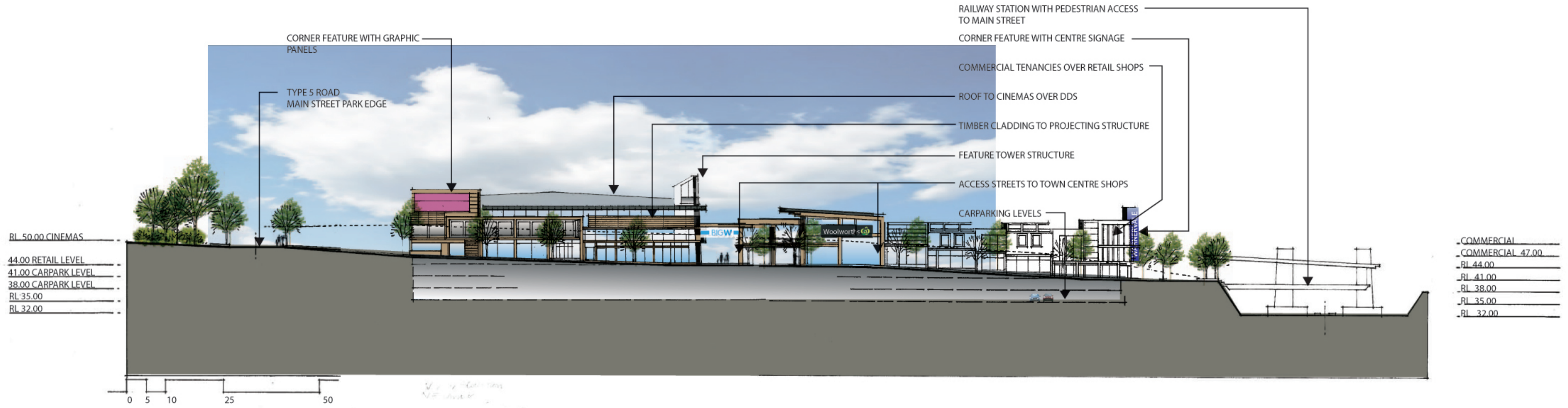
1. SOUTHERN SITE NORTH ELEVATION
