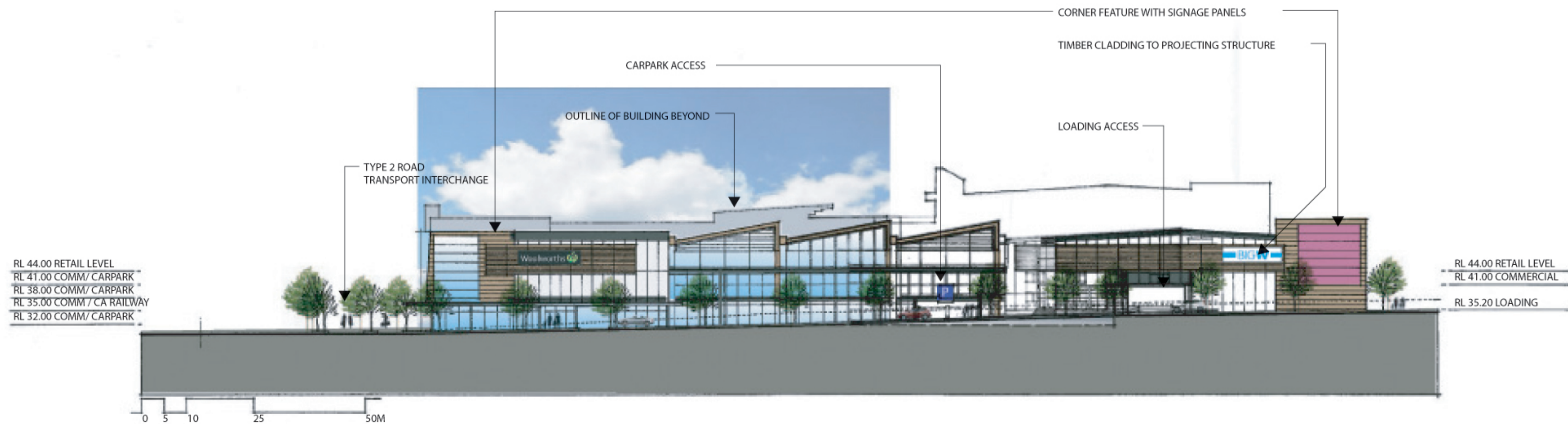
2. SOUTHERN SITE SOUTH ELEVATION
