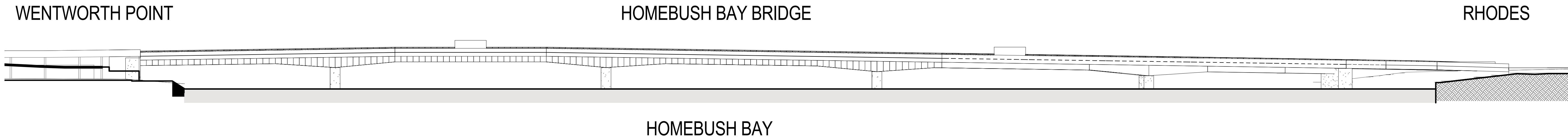
02 BRIDGE - SOUTH ELEVATION 1 : 500
