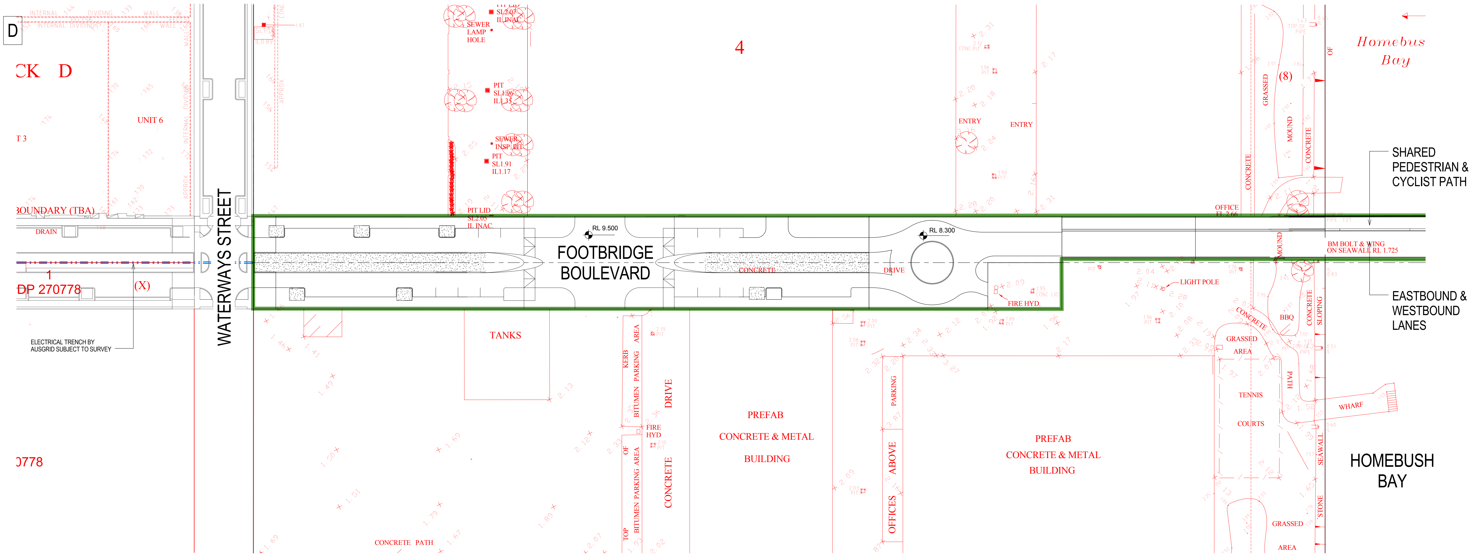
01 SITE PLAN - WENTWORTH POINT BRIDGE APPROACH 1 : 500
