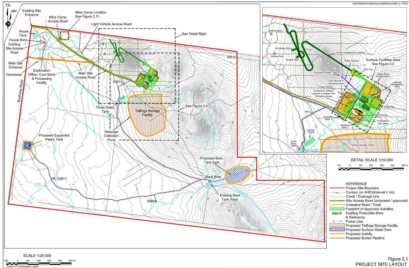
Figure 1: Mine Site Layout
